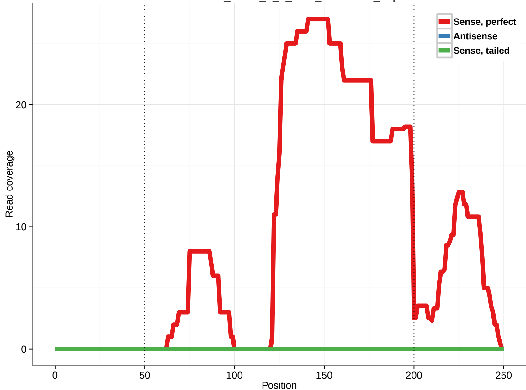
uc010oem.1_intron_8_0_chr1_24987888_f.3p
