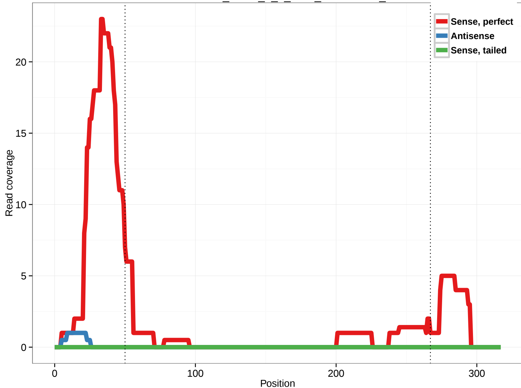
uc010nvf.2_intron_3_0_chrX_153994274_f
