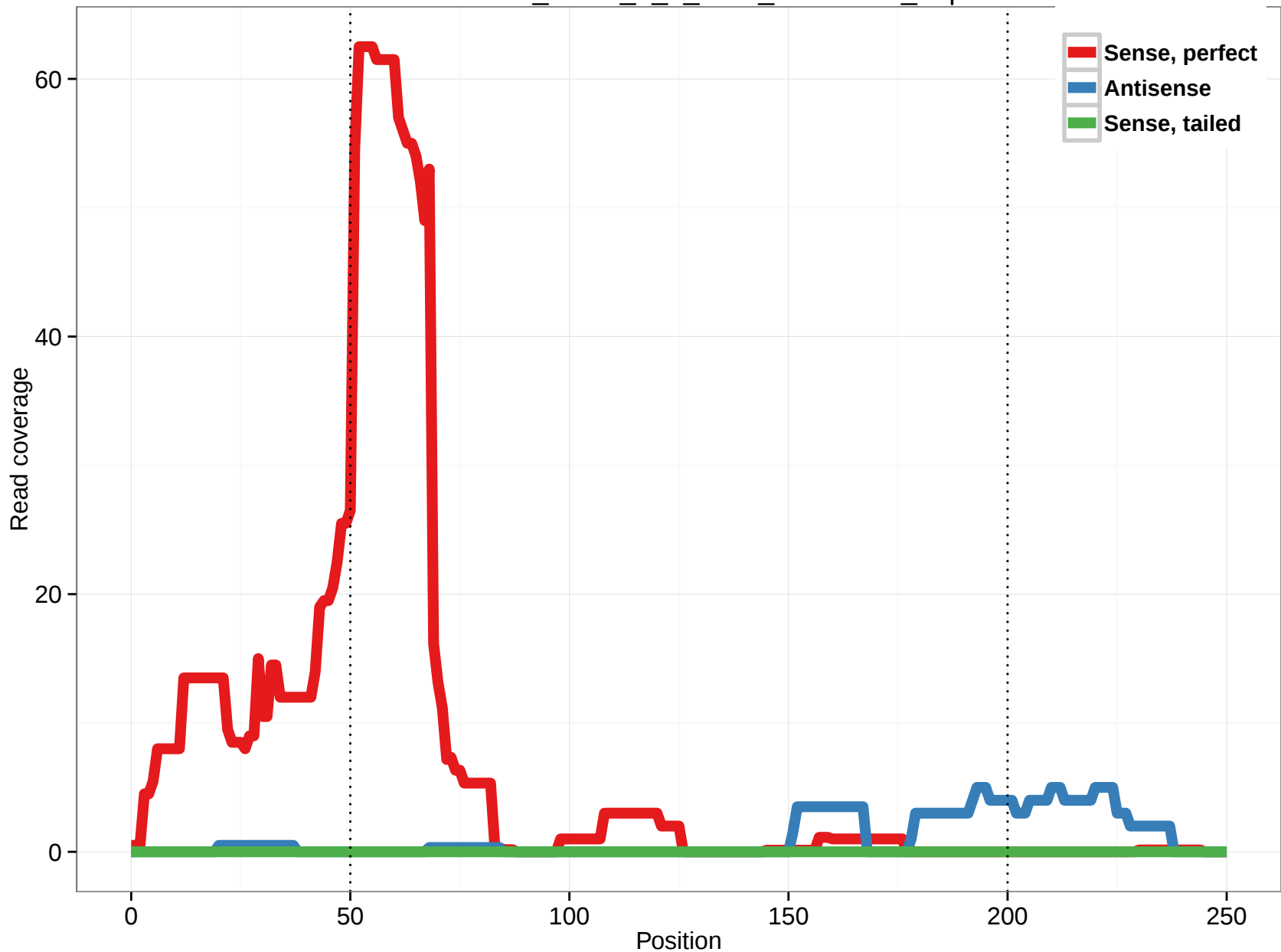
uc010nel.1_intron_3_0_chrX_13738102_r.5p
