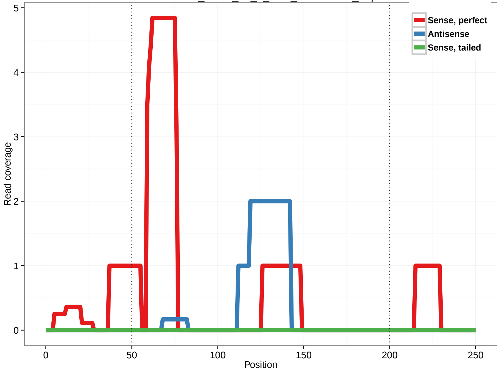
uc010ncf.1_intron_12_0_chr9_140249226_r.3p
