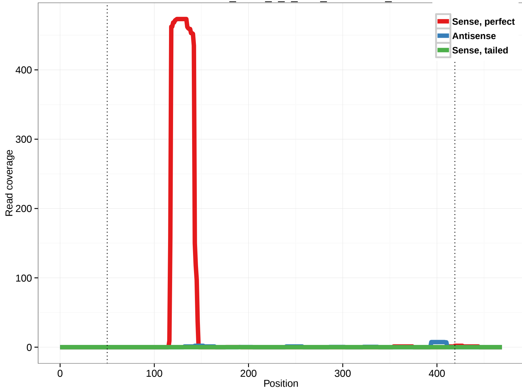
uc010mxo.2_intron_1_0_chr9_130502168_r
