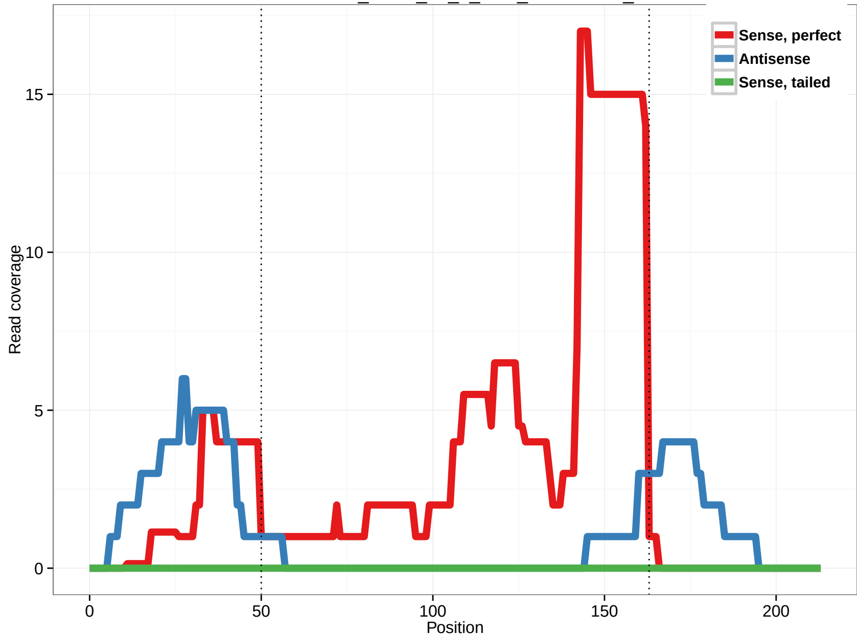
uc010lhl.1_intron_17_0_chr7_100485765_f
