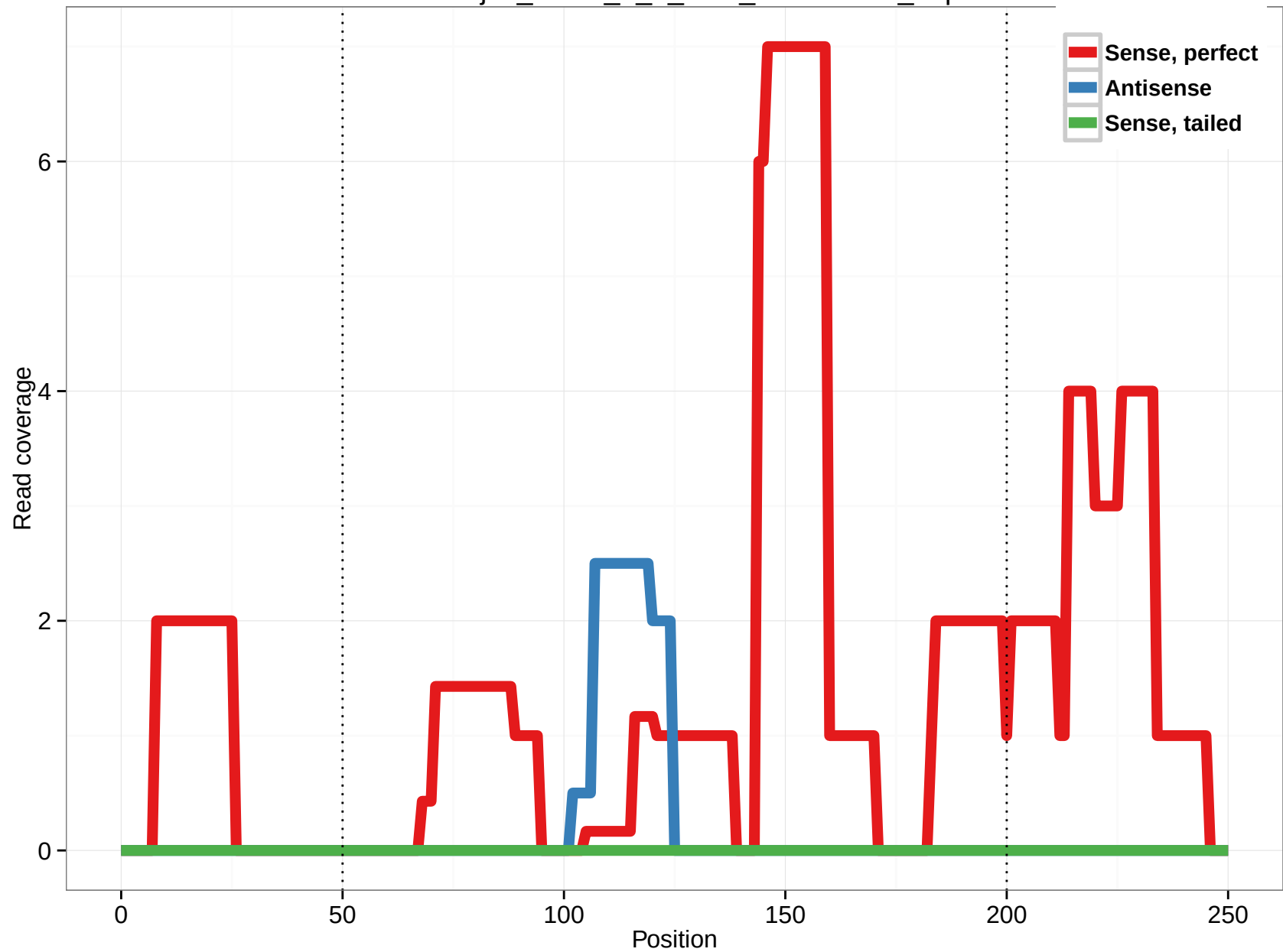
uc010kl.2_intron_1_0_chr6_157488320_f.3p
