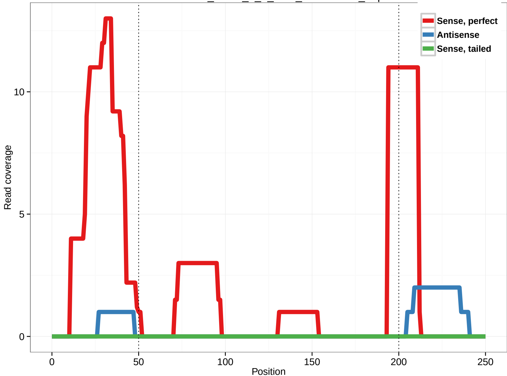
uc010kiz.2_intron_4_0_chr6_152643022_r.5p
