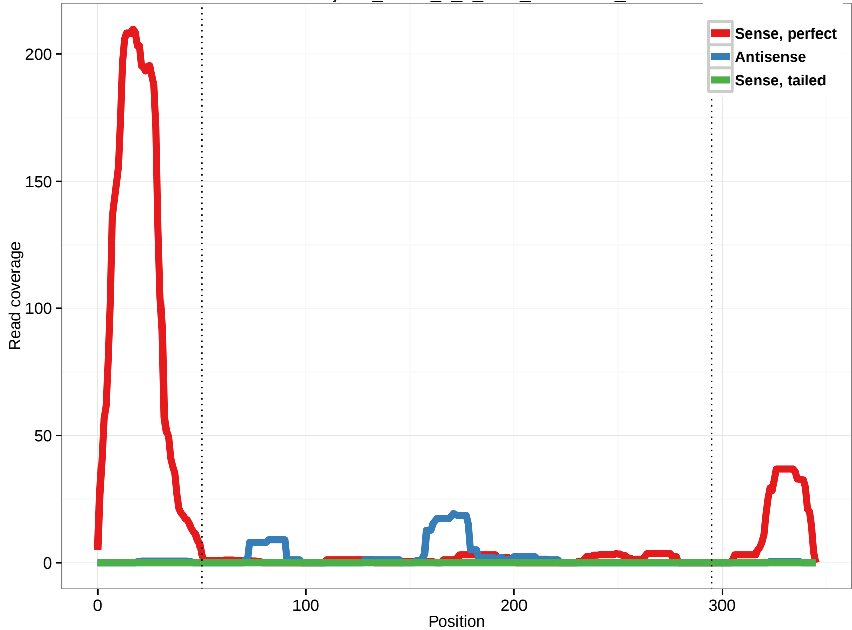
uc010jso.2_intron_0_0_chr6_31324220_r
