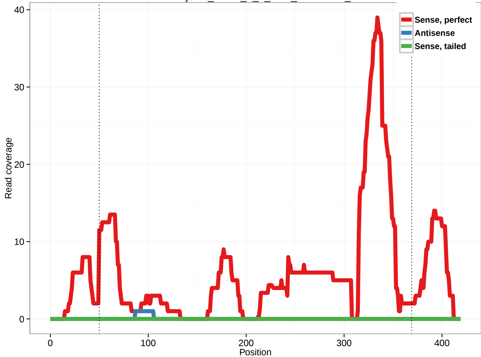
uc010jsc.1_intron_8_0_chr6_30572452_r
