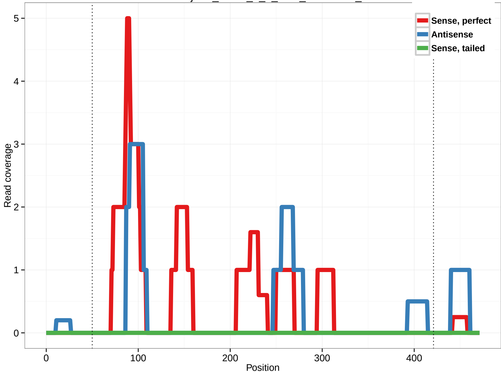
uc010jra.2_intron_6_0_chr6_28323452_r
