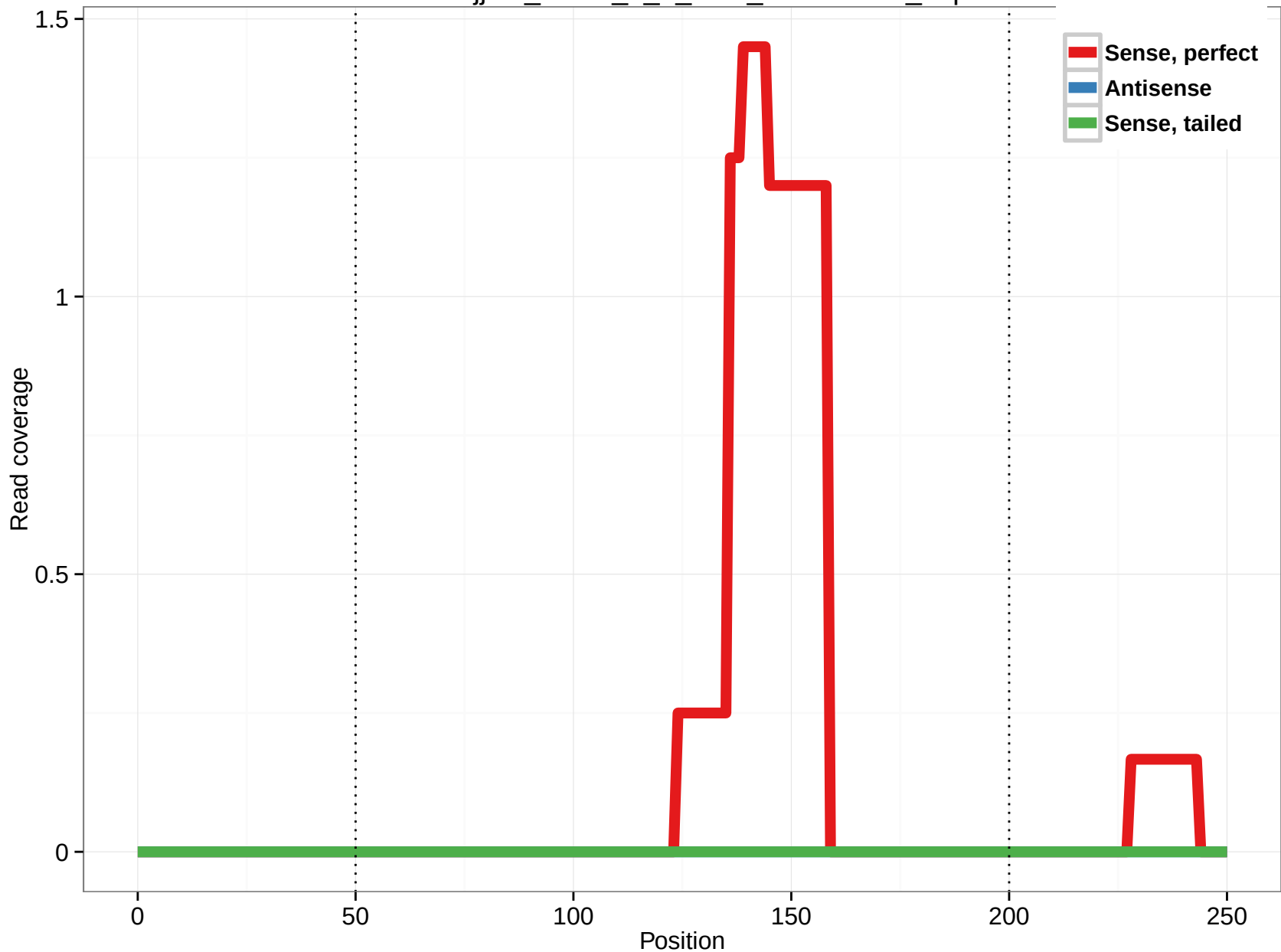
uc010jjc.2_intron_8_0_chr5_161576320_f.3p
