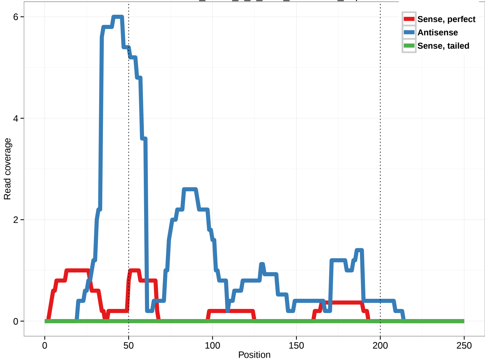
uc010ixz.1_intron_3_0_chr5_69771428_f.5p
