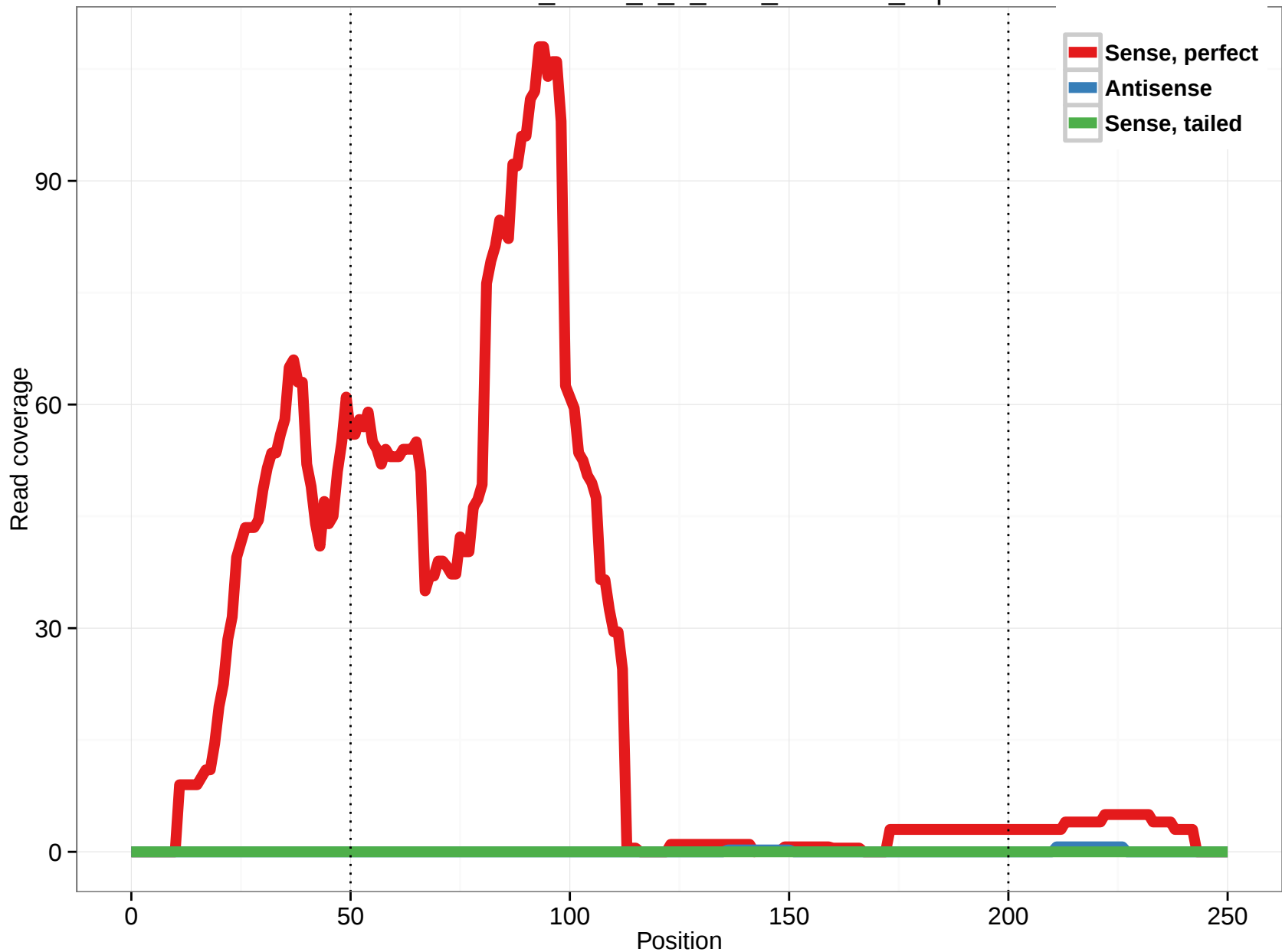
uc010itn.1_intron_0_0_chr5_7869303_f.5p
