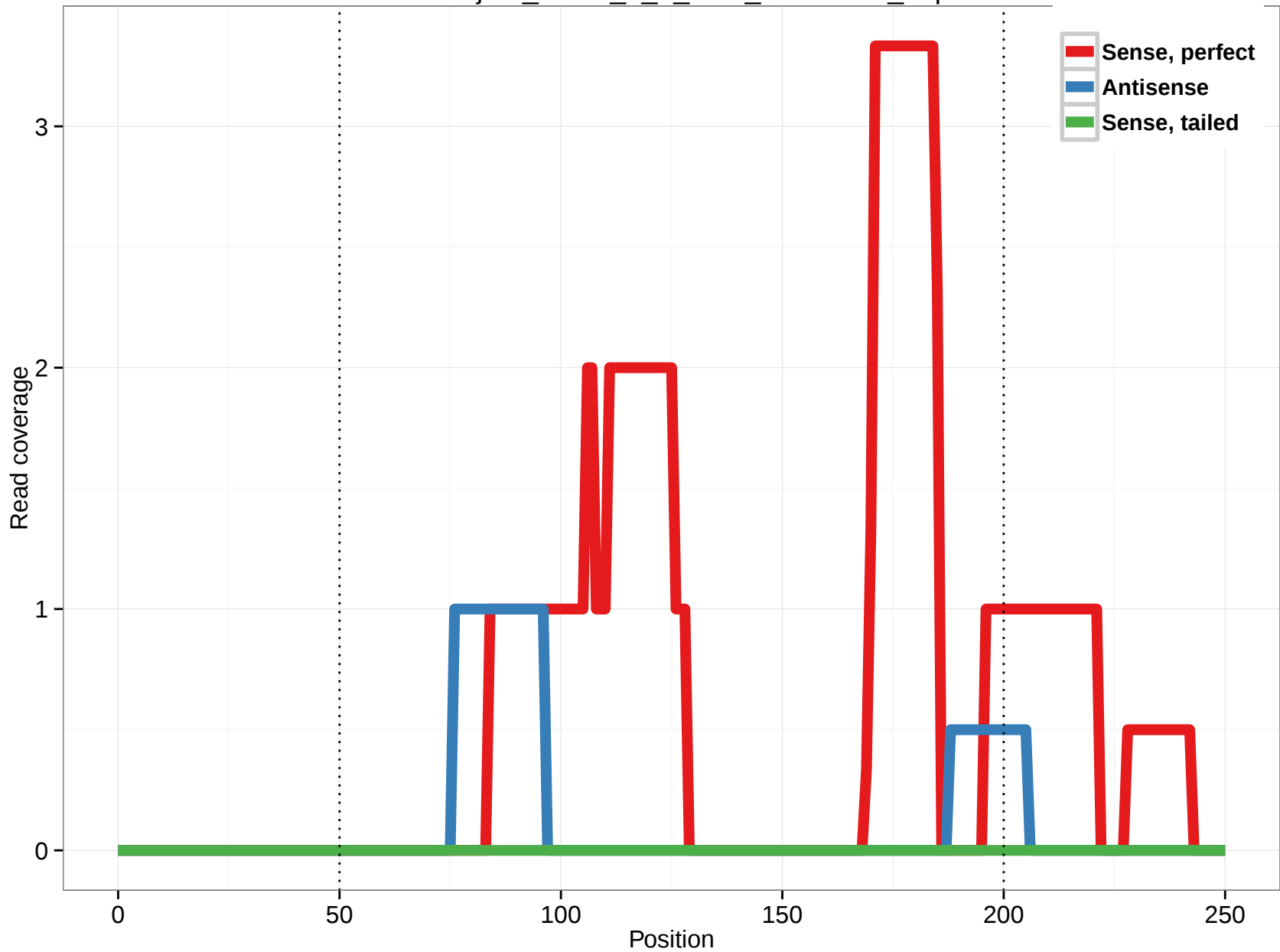
uc010ijh.1_intron_2_0_chr4_77894224_f.5p
