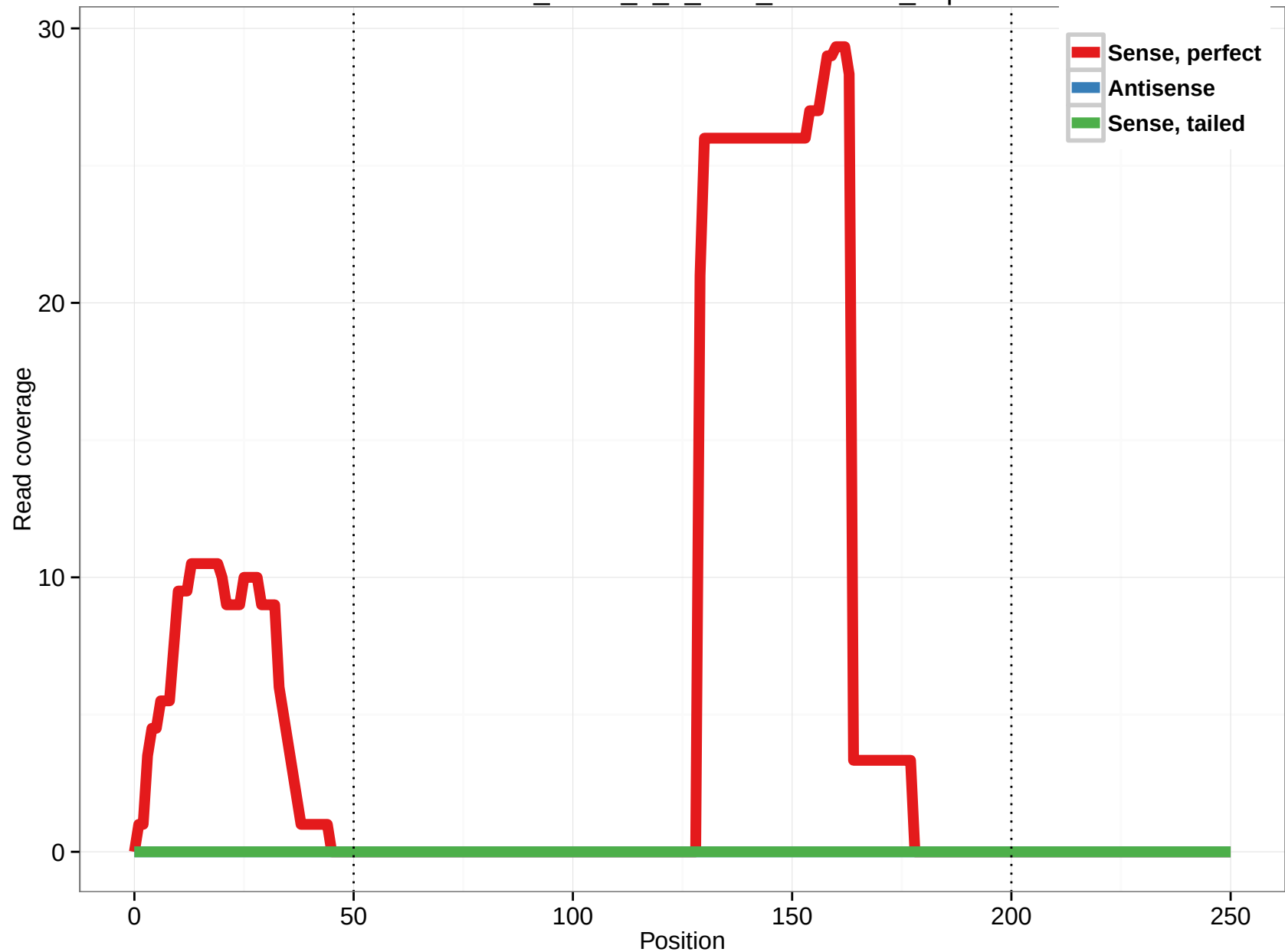
uc010ihf.2_intron_1_0_chr4_57786037_f.5p
