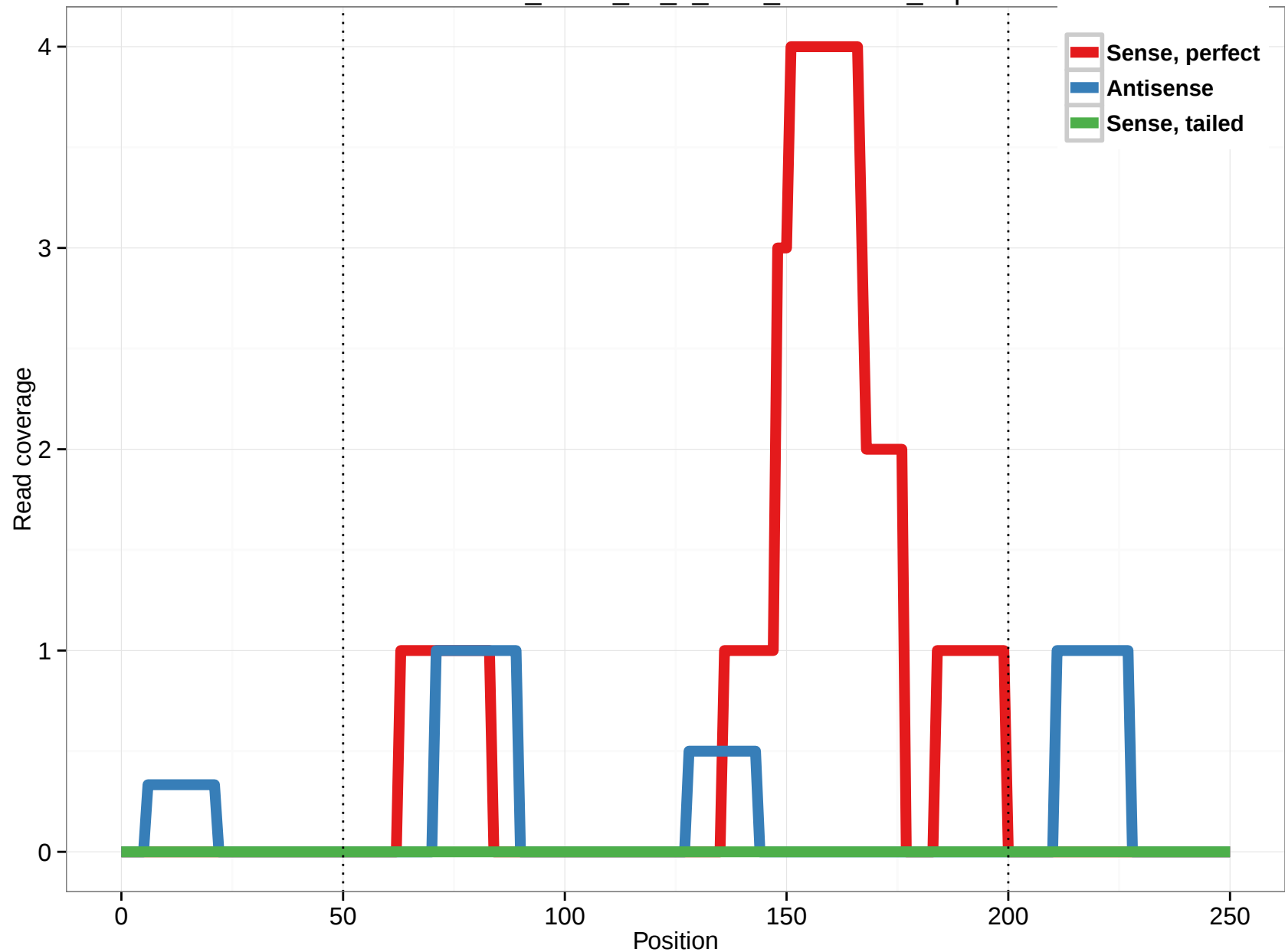
uc010iew.2_intron_18_0_chr4_26750149_f.3p
