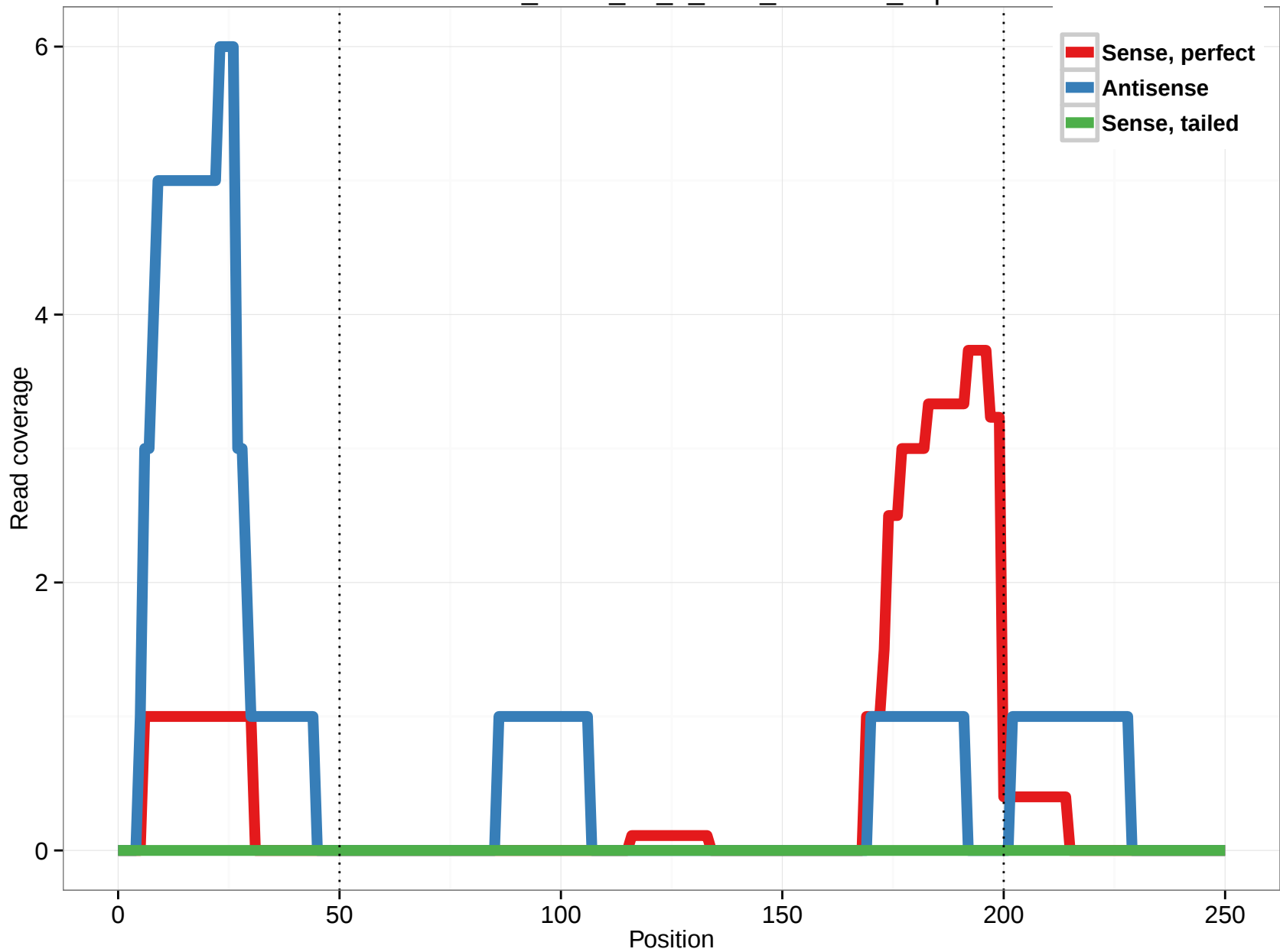
uc010icl.2_intron_16_0_chr4_2702272_f.3p
