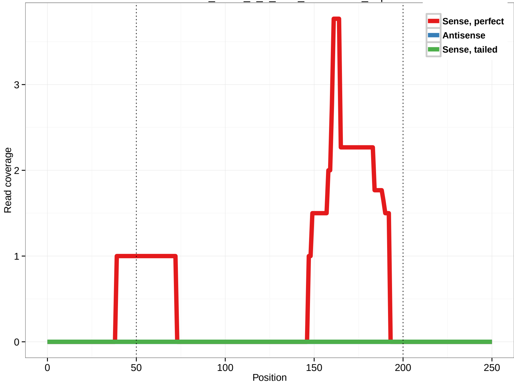
uc010hvr.1_intron_9_0_chr3_154858082_f.5p
