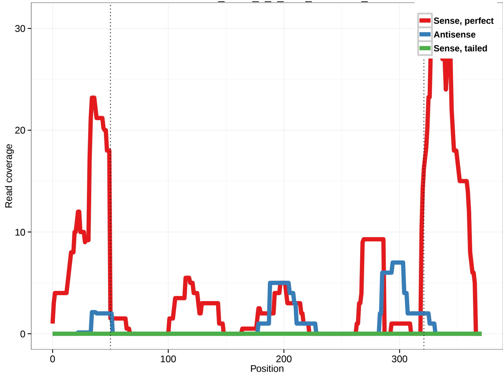
uc010hia.1_intron_9_0_chr3_41275359_f
