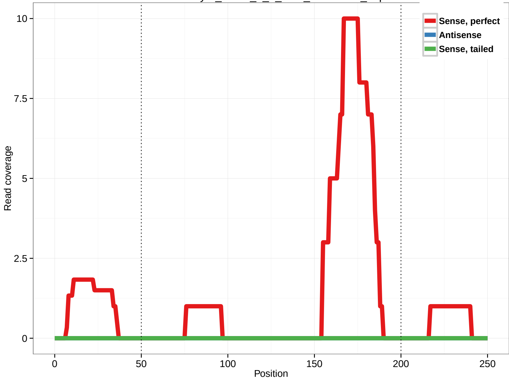
uc010hey.2_intron_2_0_chr3_20012210_f.5p
