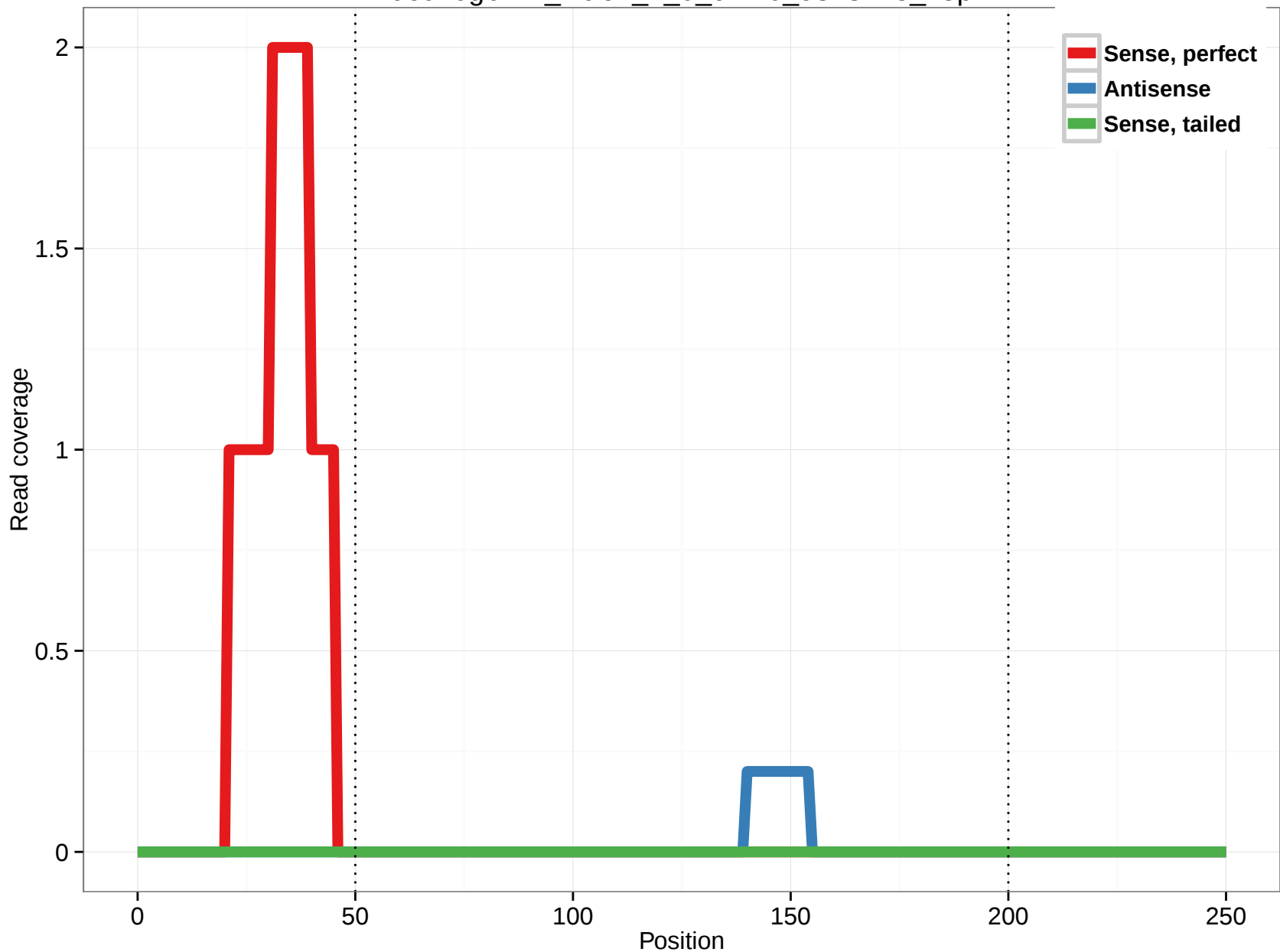
uc010gbw.1_intron_4_0_chr20_9318715_f.5p
