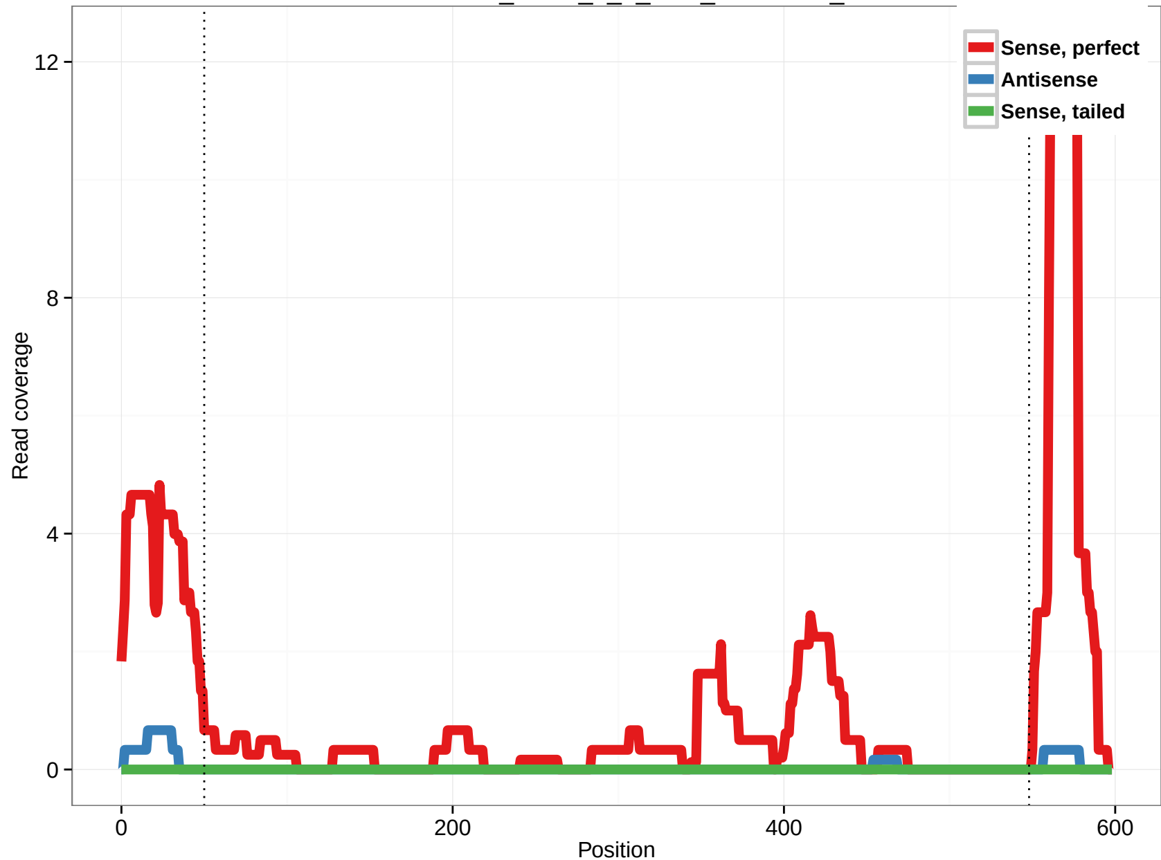
uc010fid.1_intron_1_0_chr2_98123529_r
