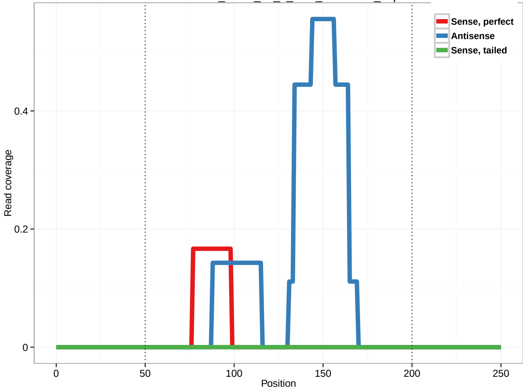
uc010fhm.2_intron_29_0_chr2_90260251_f.3p
