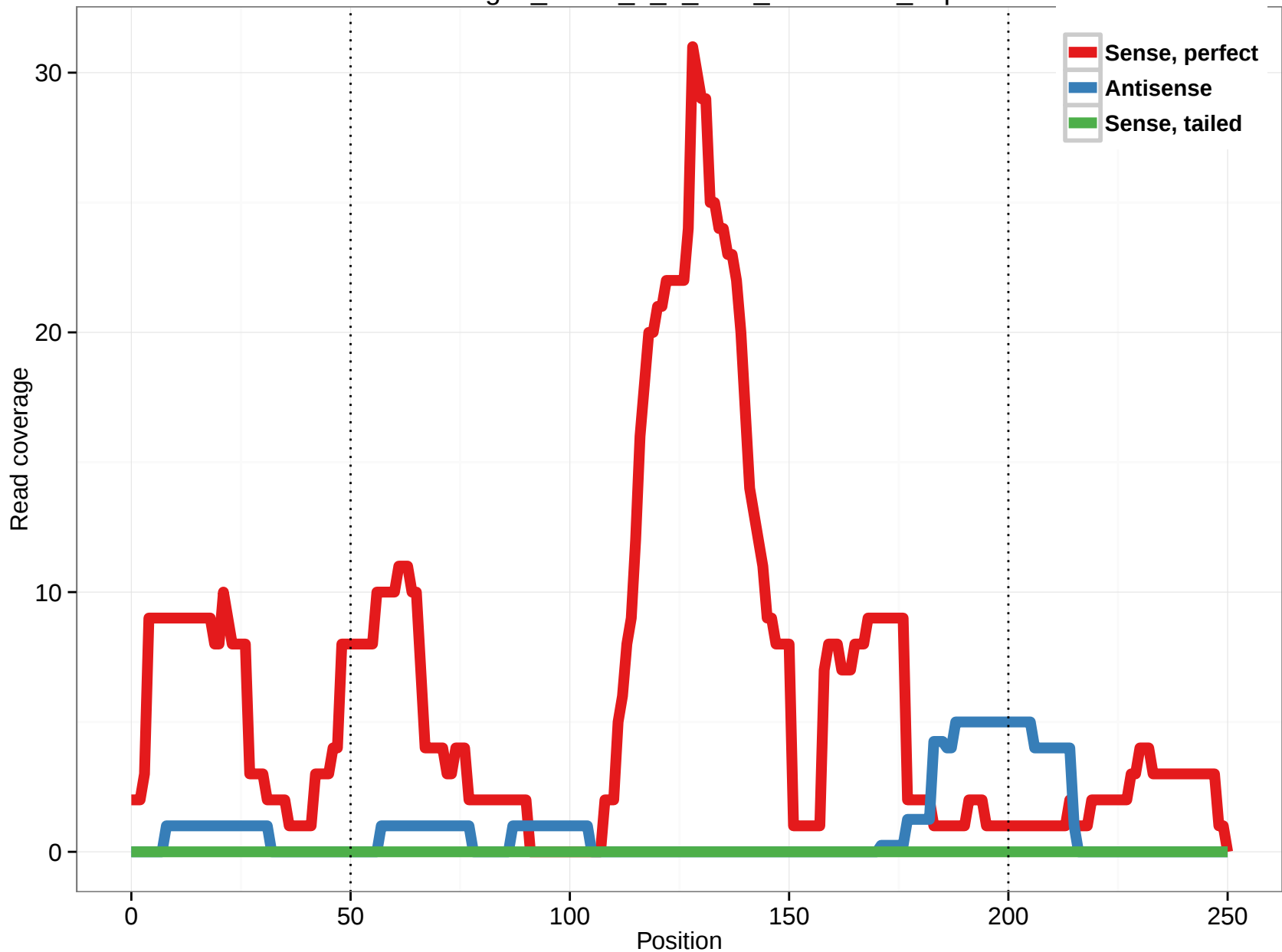
uc010fgl.2_intron_0_0_chr2_85767124_f.5p
