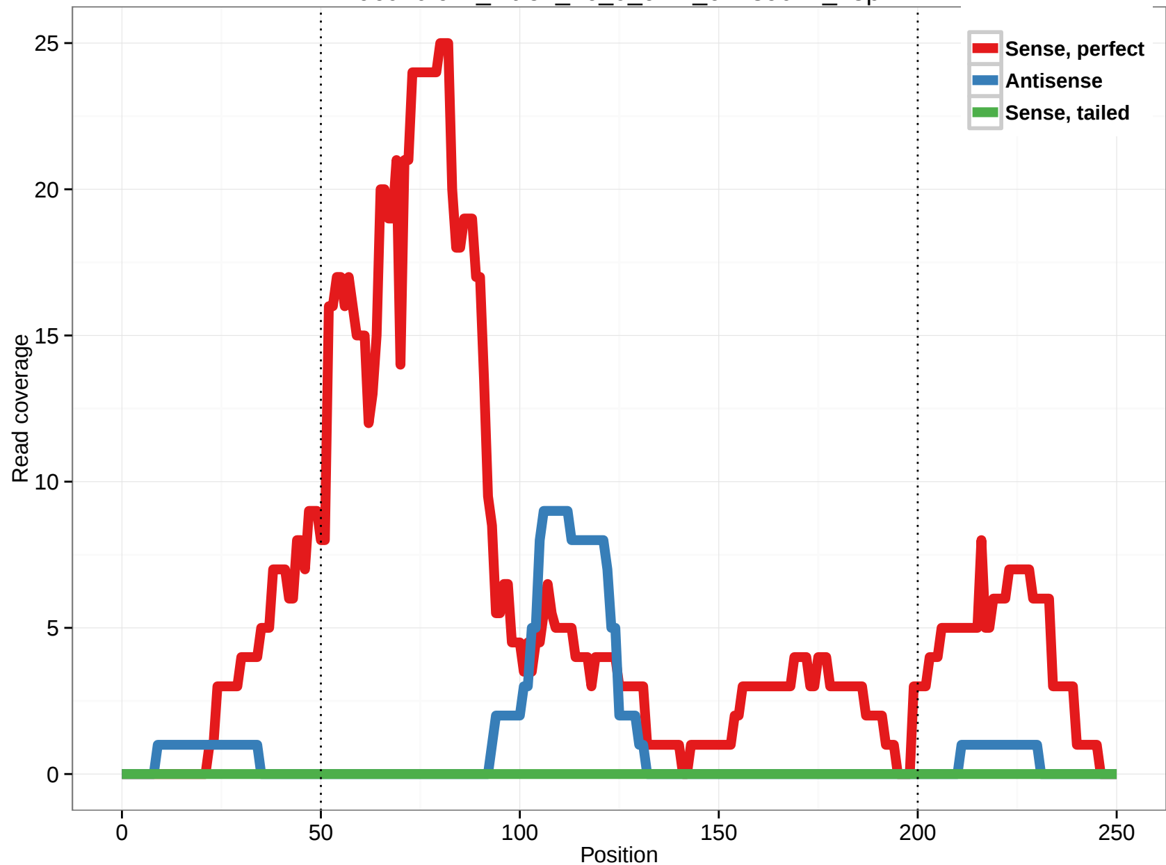
uc010fci.2_intron_16_0_chr2_61239041_r.5p
