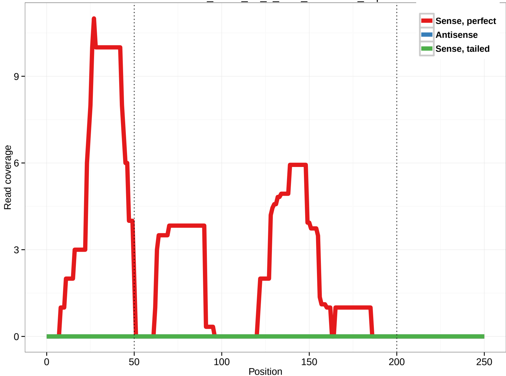
uc010ezu.2_intron_25_0_chr2_32690233_f.5p
