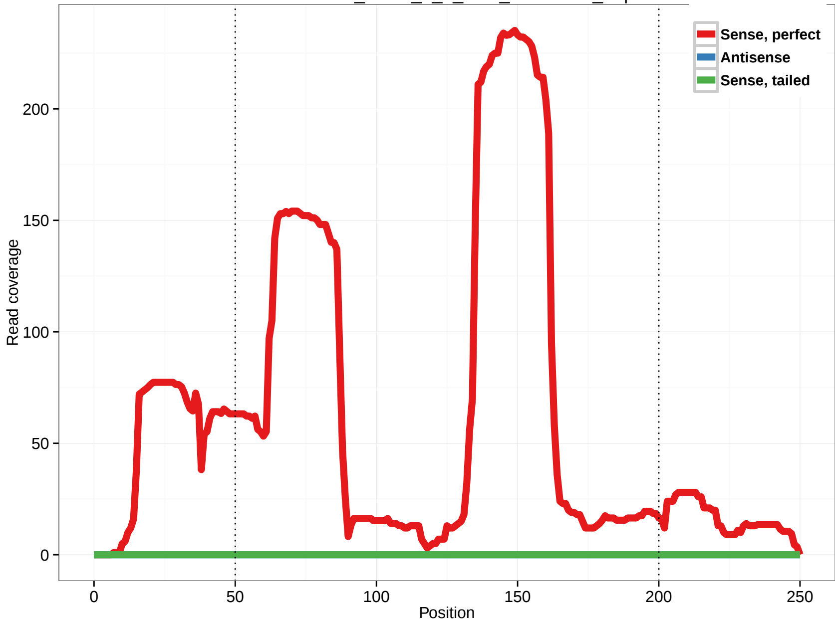
uc010exv.2_intron_0_0_chr2_20402063_r.3p
