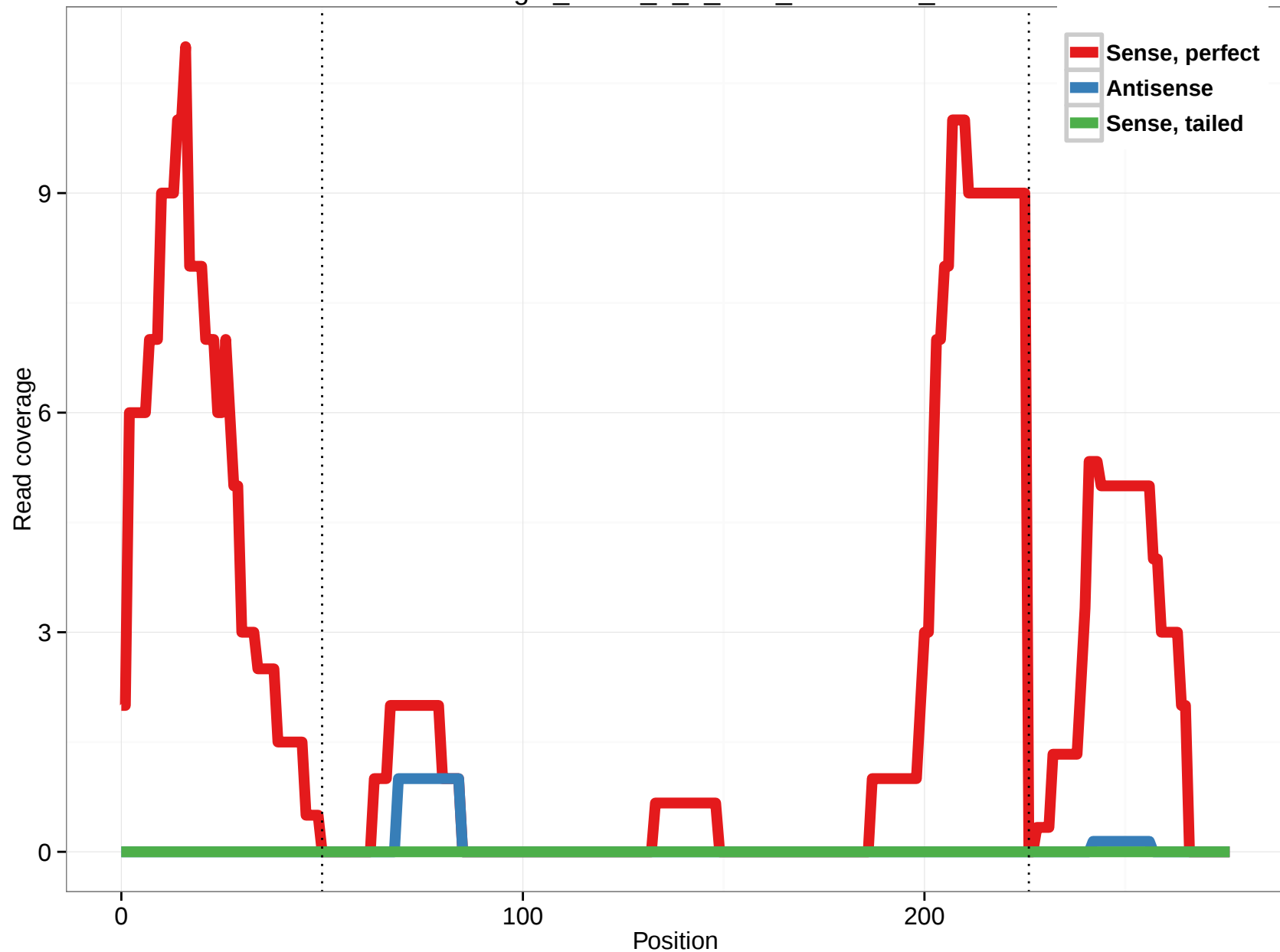
uc010exg.1_intron_4_0_chr2_10583440_r
