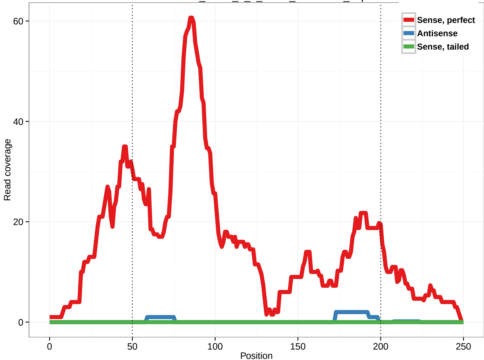
uc010eet.2_intron_0_0_chr19_36706058_f.5p
