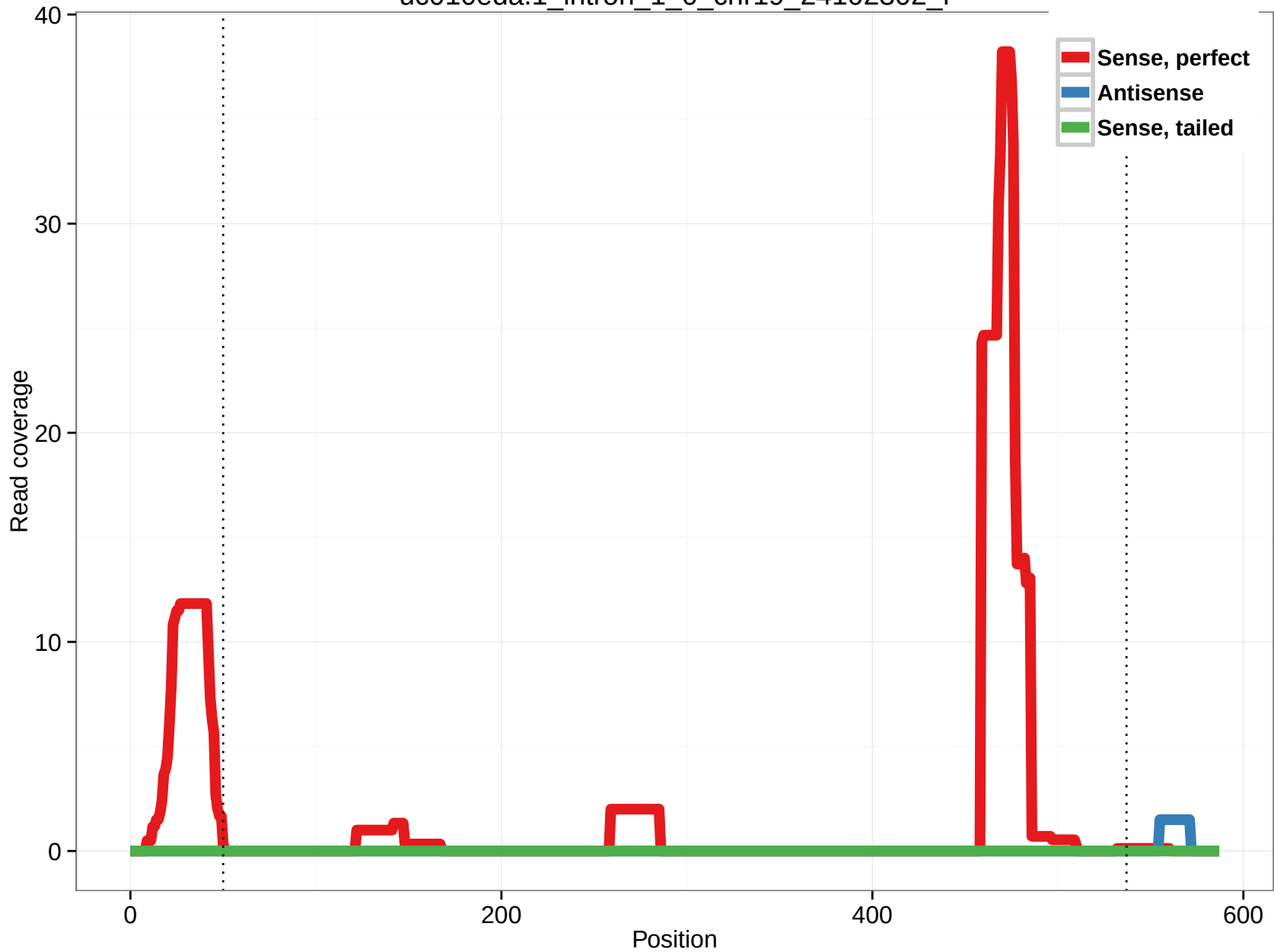
uc010eda.1_intron_1_0_chr19_24102302_f
