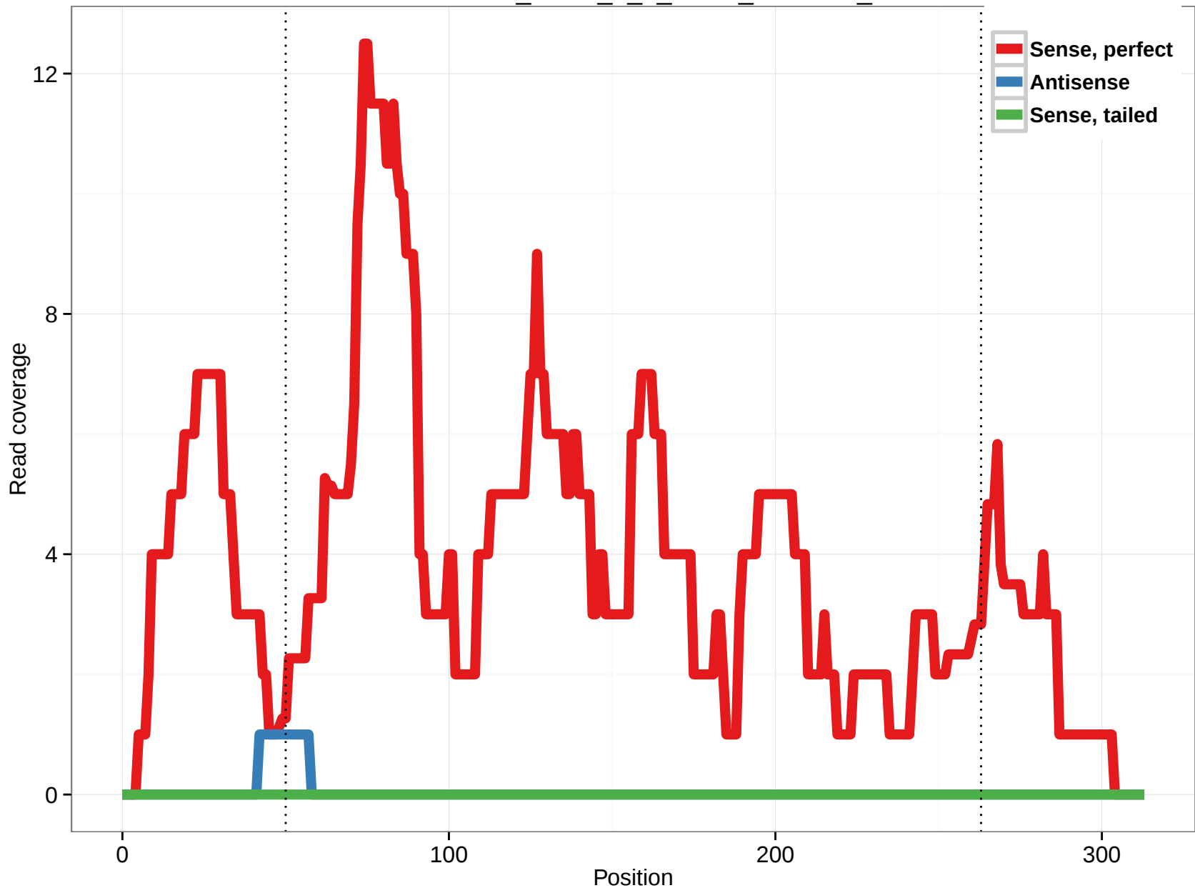
uc010dtc.1_intron_0_0_chr19_2429487_r
