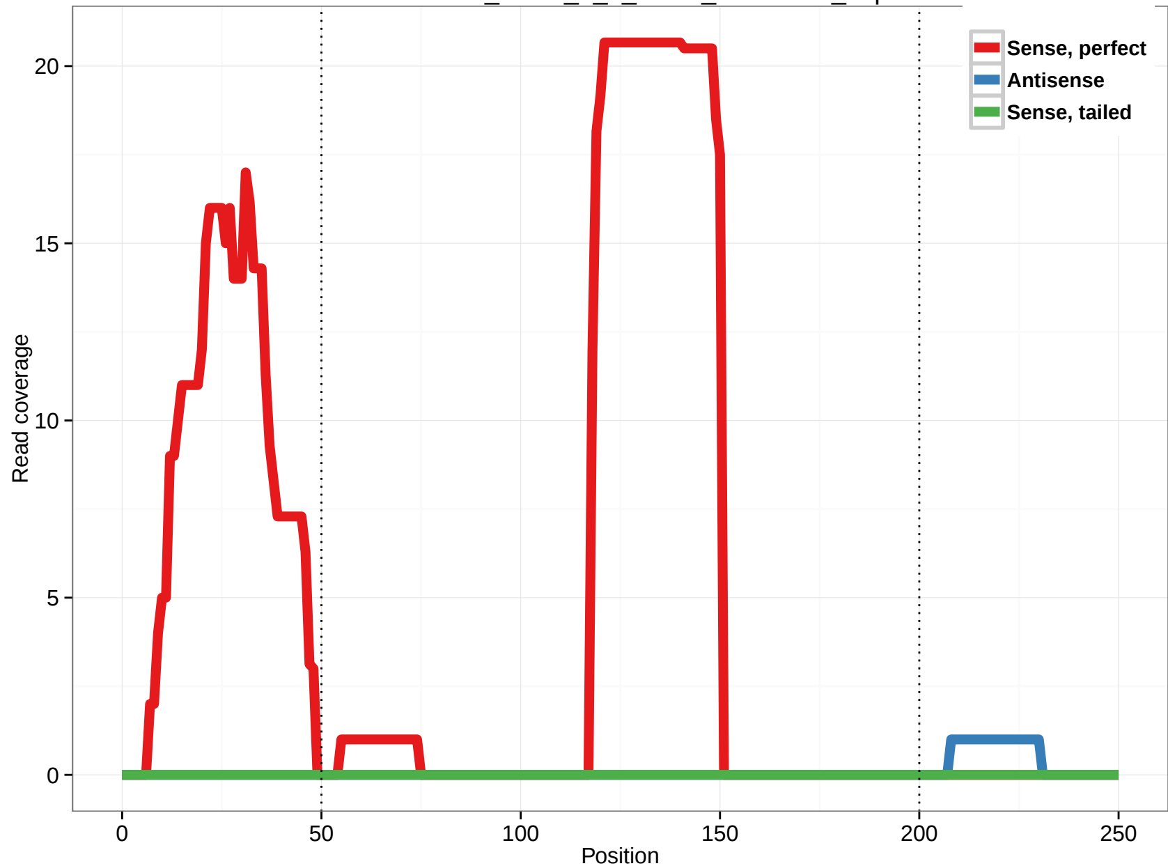
uc010czd.2_intron_5_0_chr17_41338462_f.5p
