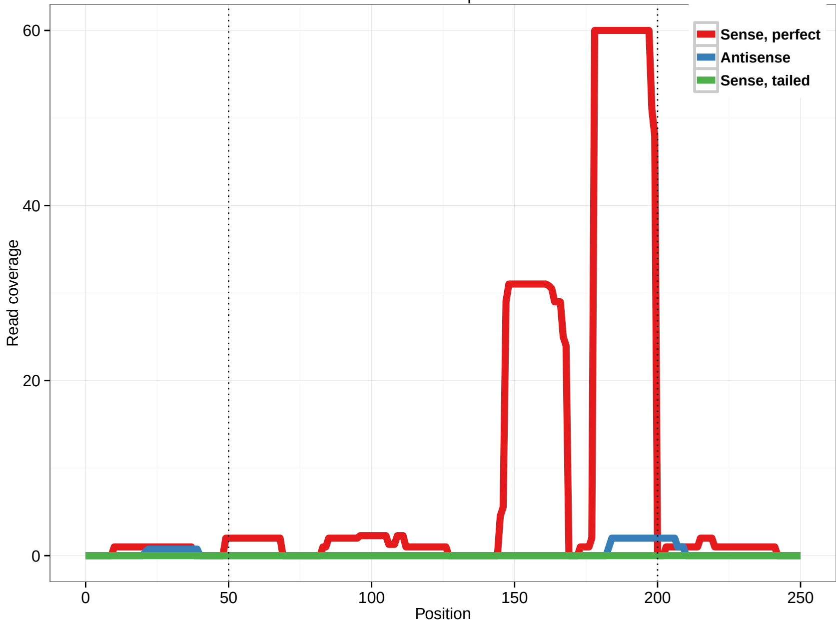
uc010cwp.5
