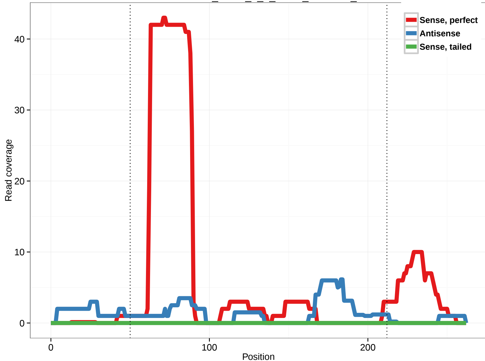
uc010cku.1_intron_2_0_chr17_4872633_r
