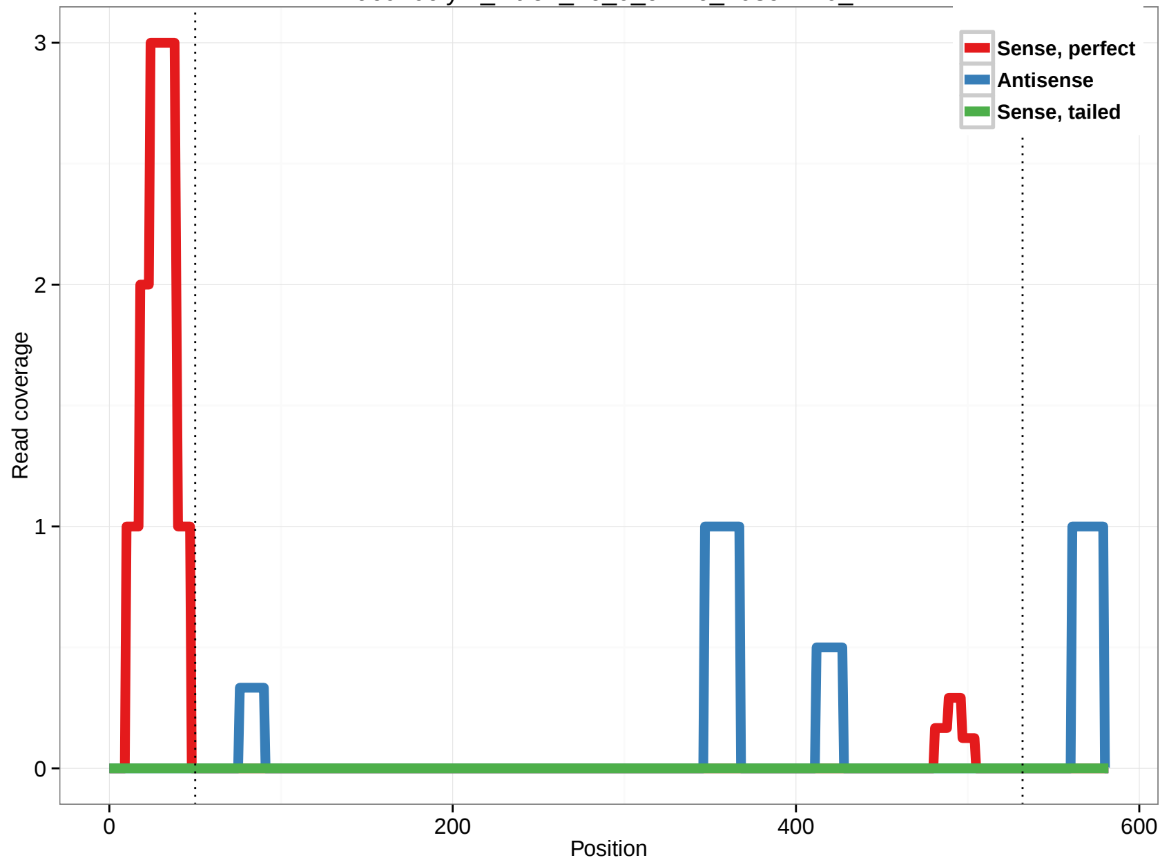
uc010cfy.2_intron_16_0_chr16_70894110_r
