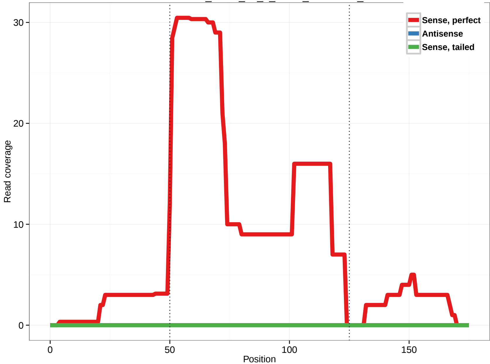
uc010cel.1_intron_24_0_chr16_67685749_f
