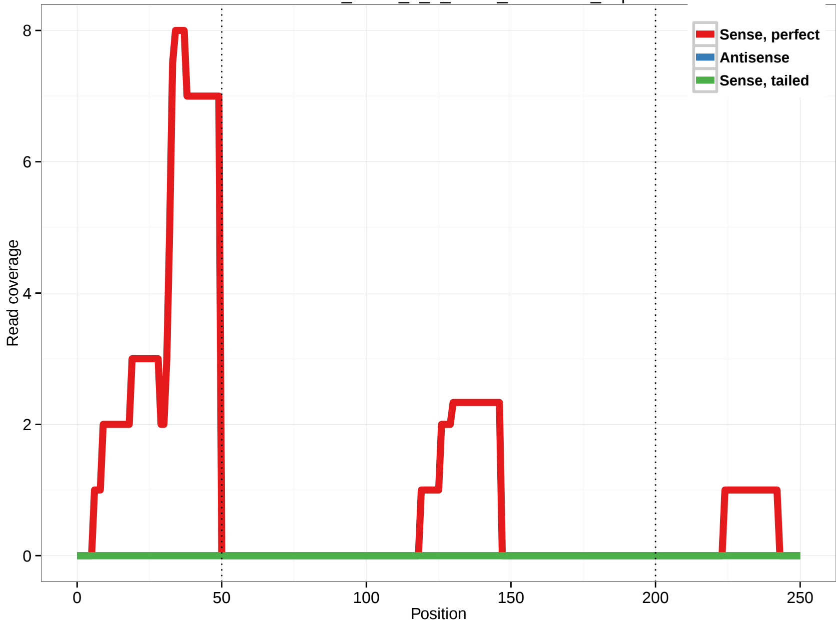
uc010bvn.2_intron_2_0_chr16_16127028_f.5p
