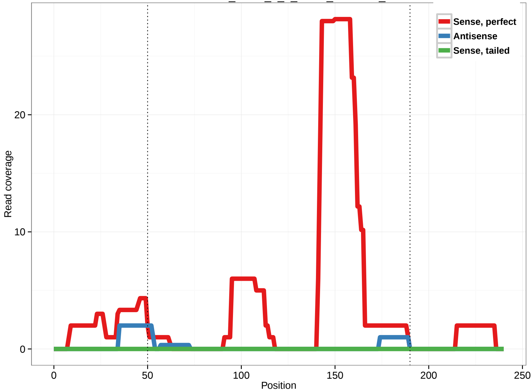
uc010bse.1_intron_2_0_chr16_2141908_r
