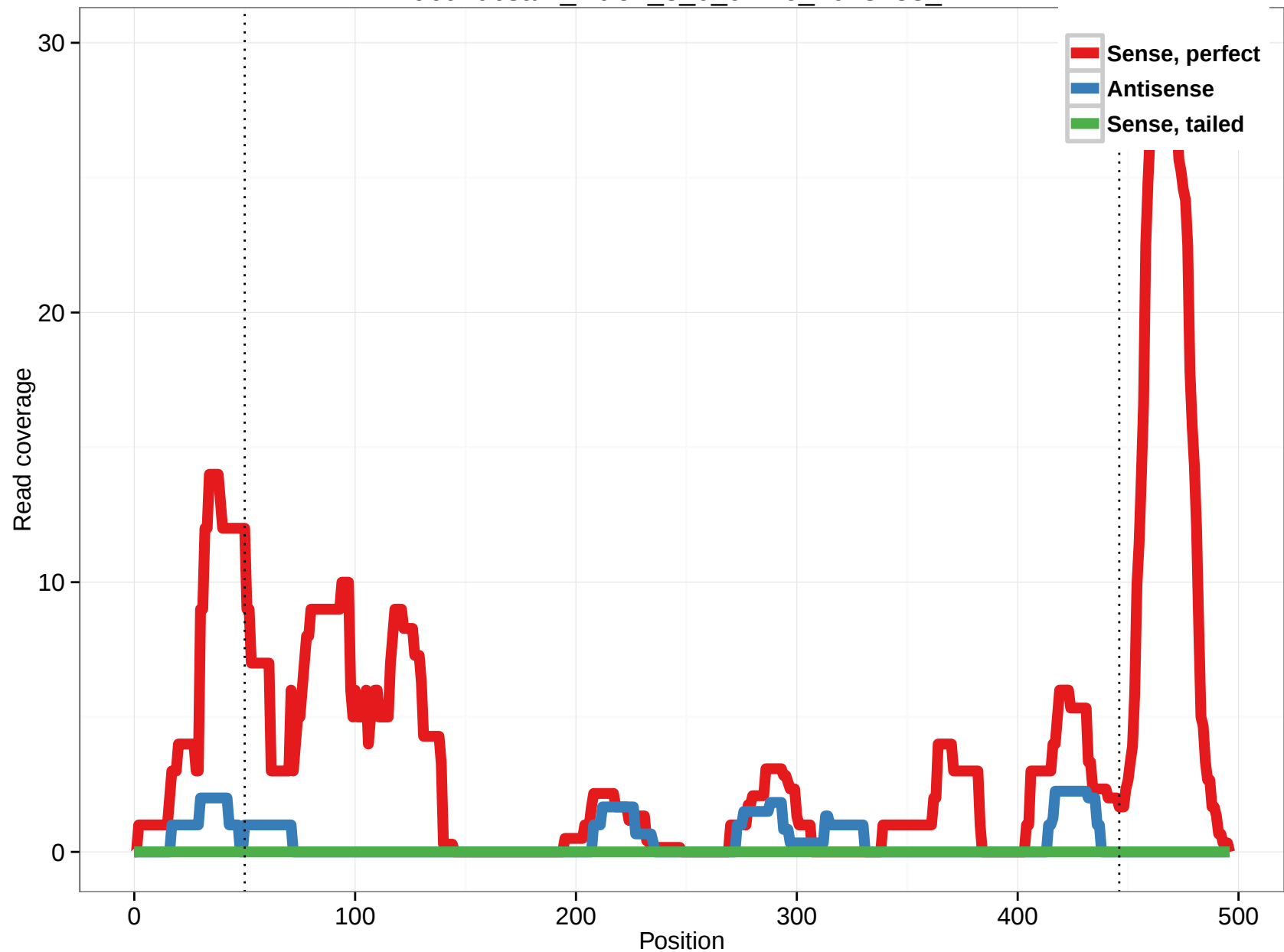
uc010bsa.1_intron_3_0_chr16_2013258_r
