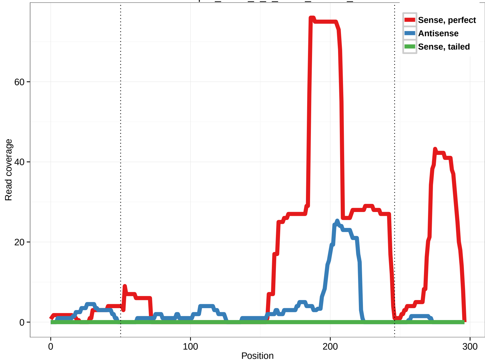
uc010bqz.2_intron_2_0_chr16_731597_f
