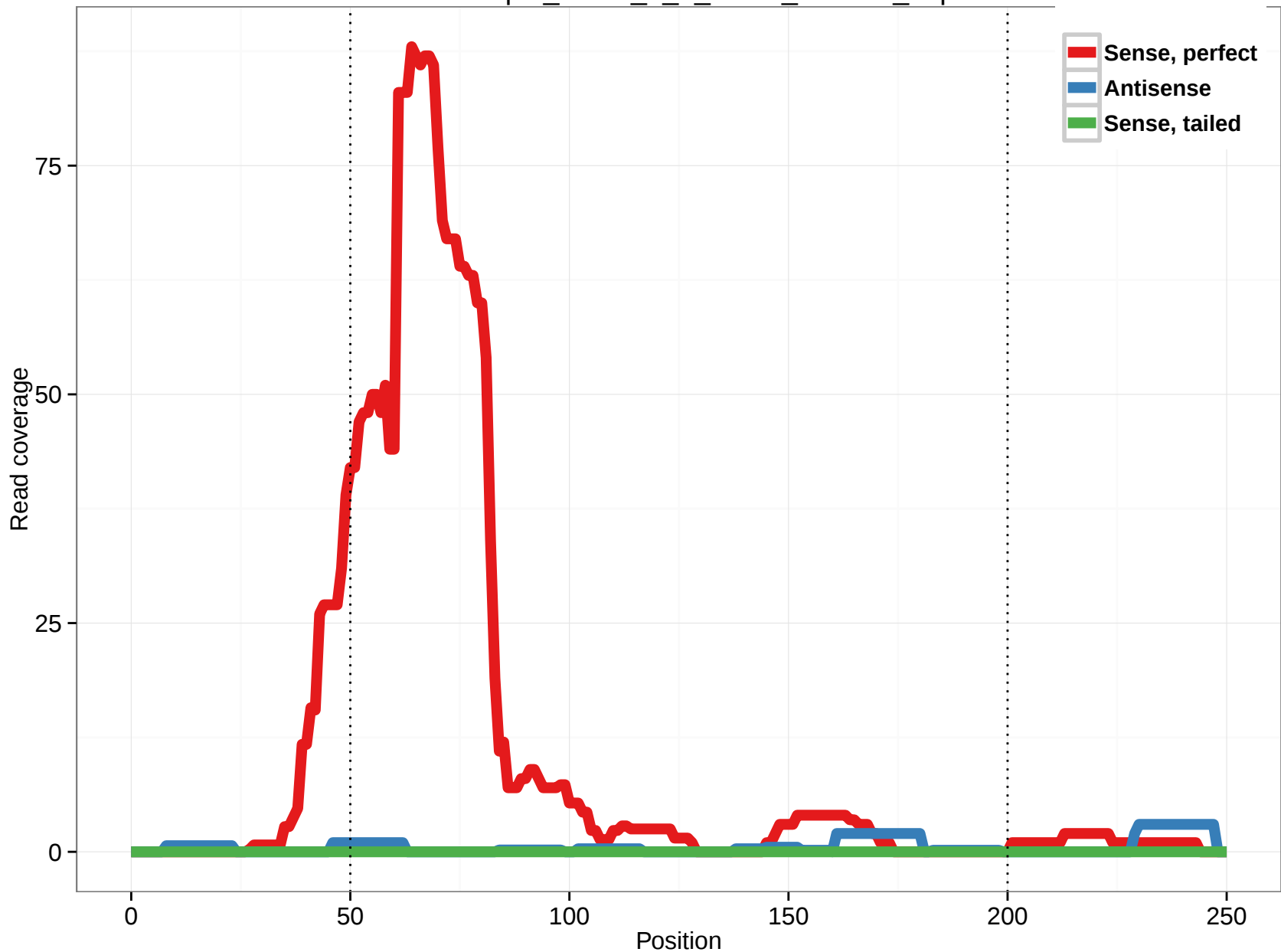
uc010bqr.2_intron_0_0_chr16_284857_f.5p
