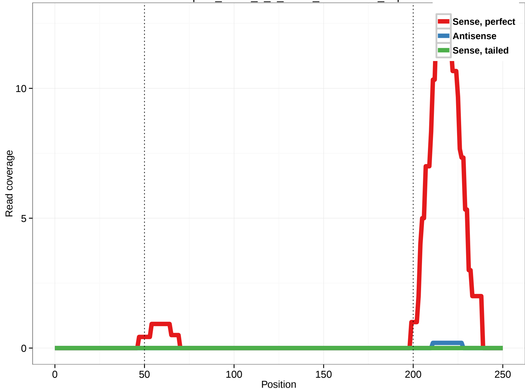
uc010bpa.1_intron_1_0_chr15_101425577_f.3p
