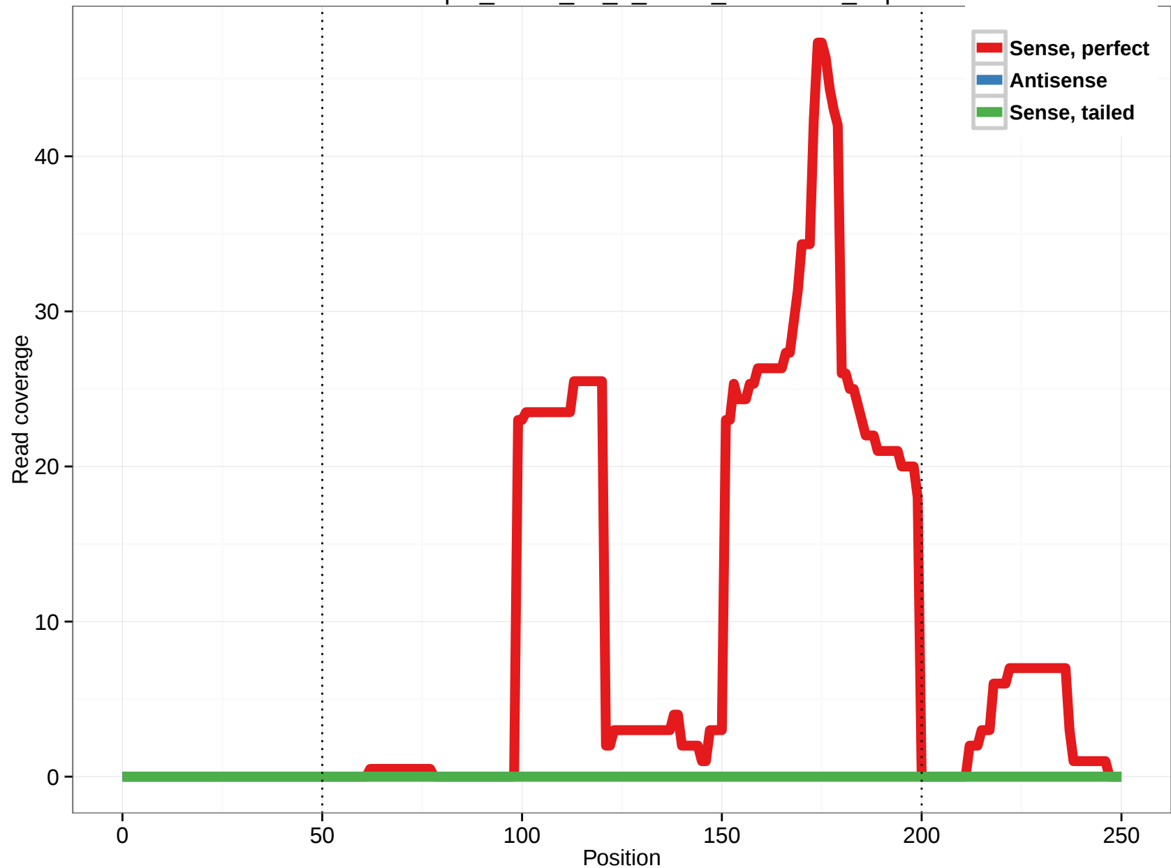
uc010bnp.1_intron_10_0_chr15_89816701_f.3p
