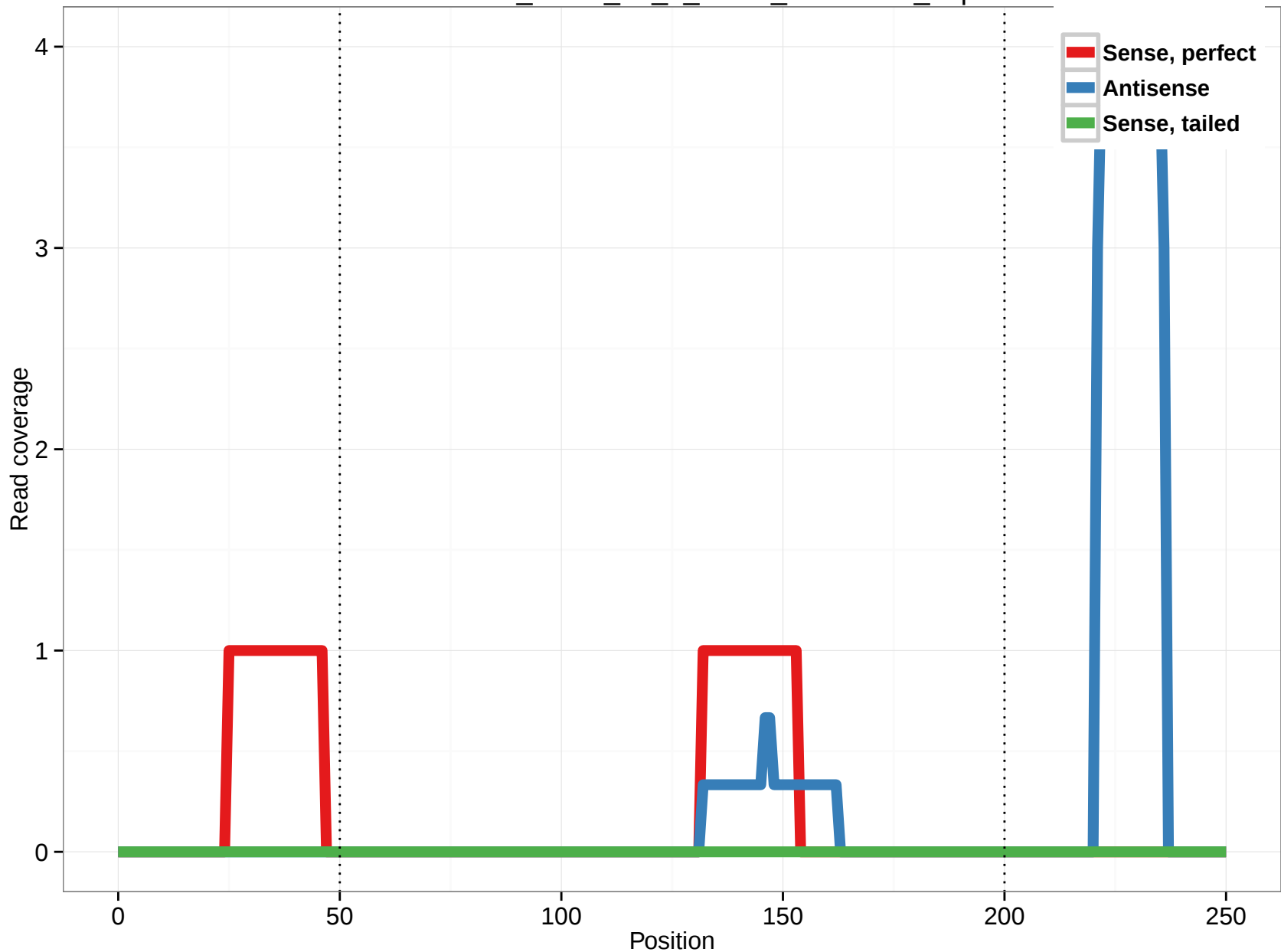
uc010bmt.1_intron_23_0_chr15_84683477_f.5p
