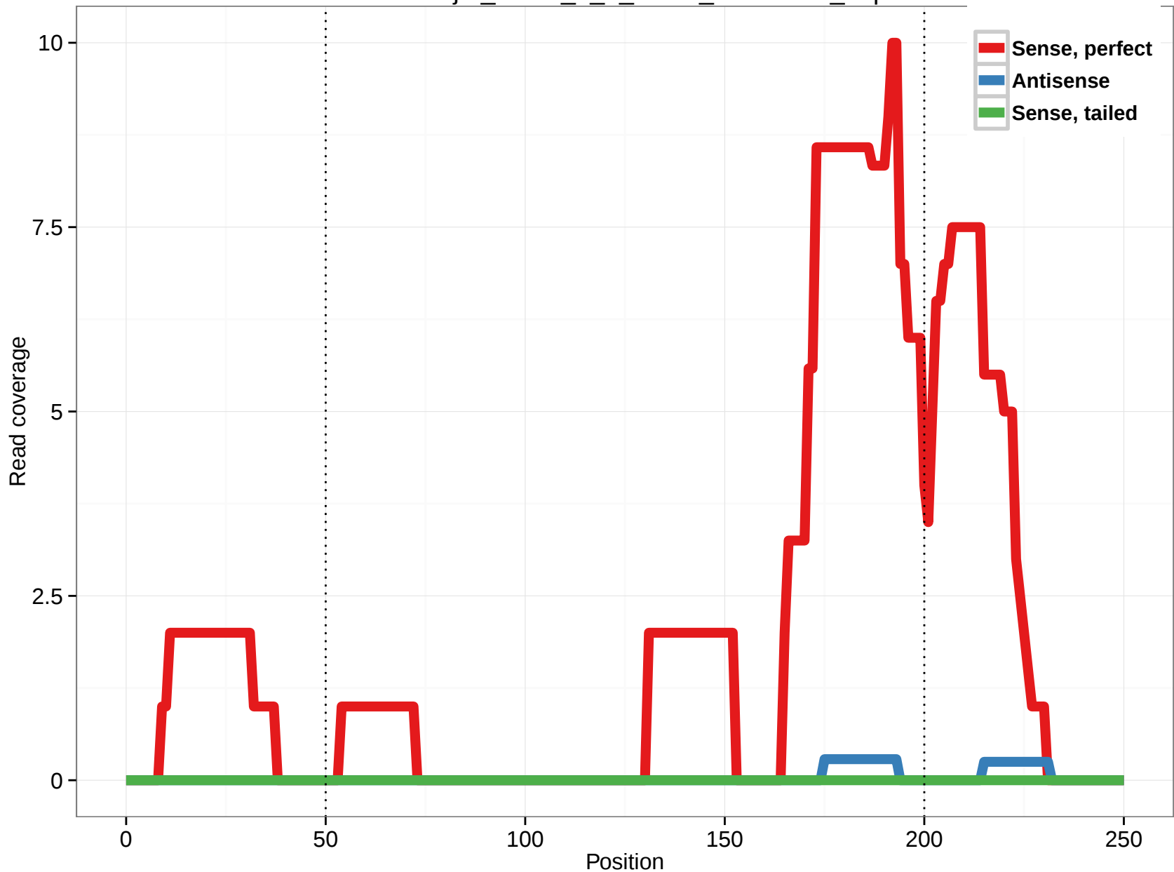
uc010blj.1_intron_3_0_chr15_79178570_f.3p
