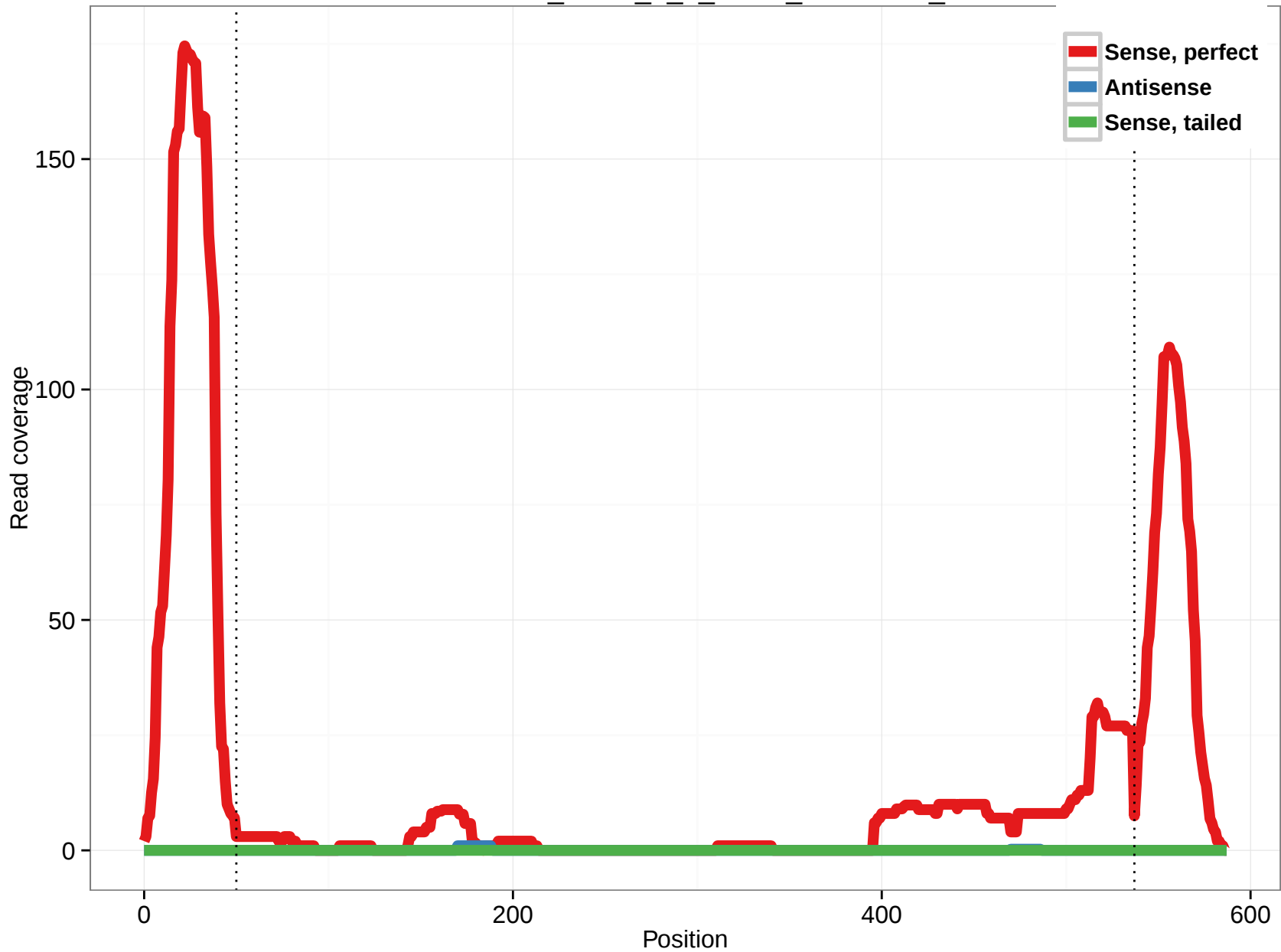
uc010bit.1_intron_6_0_chr15_72502201_r
