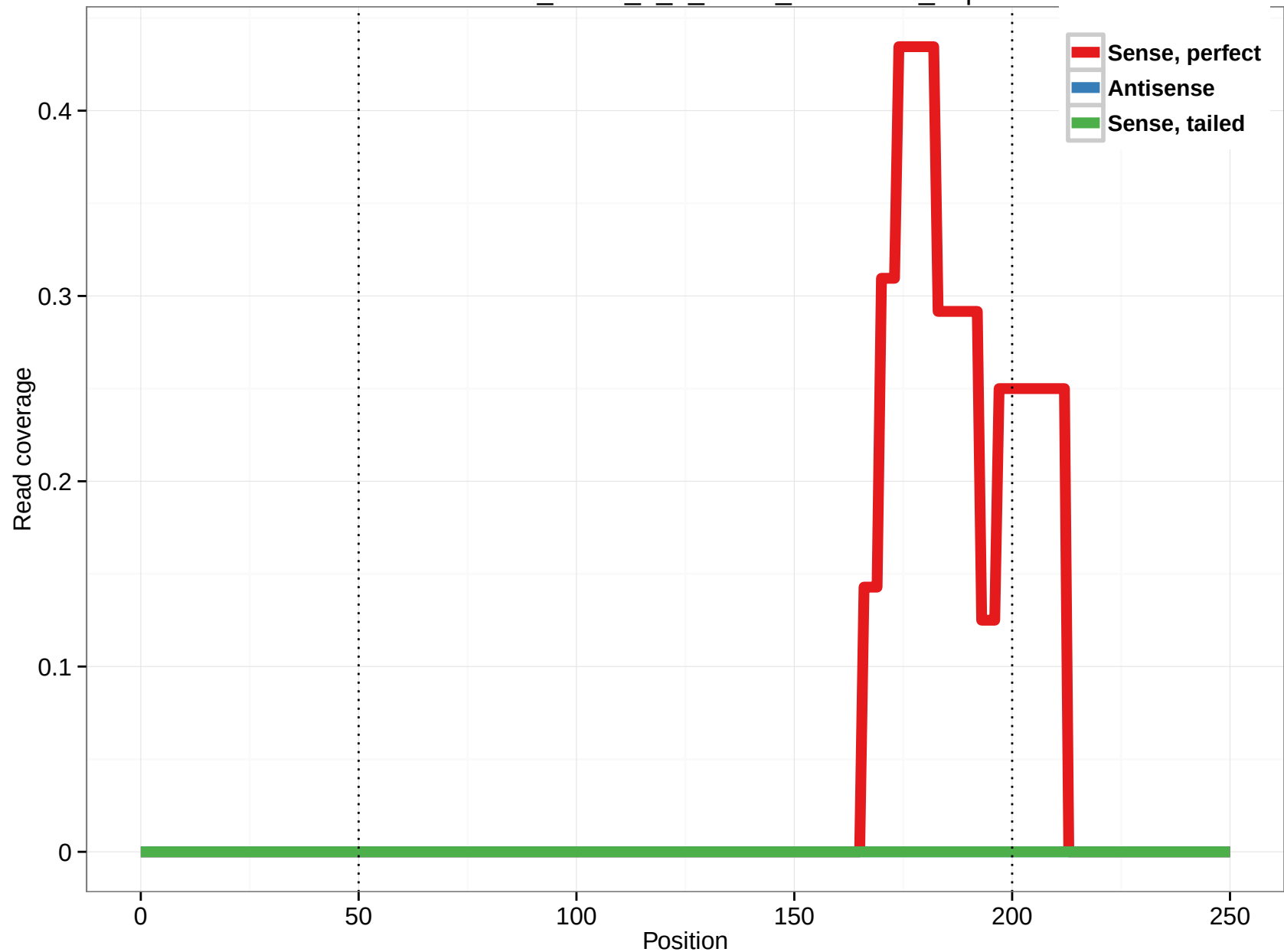
uc010bab.1_intron_1_0_chr15_32323241_f.3p
