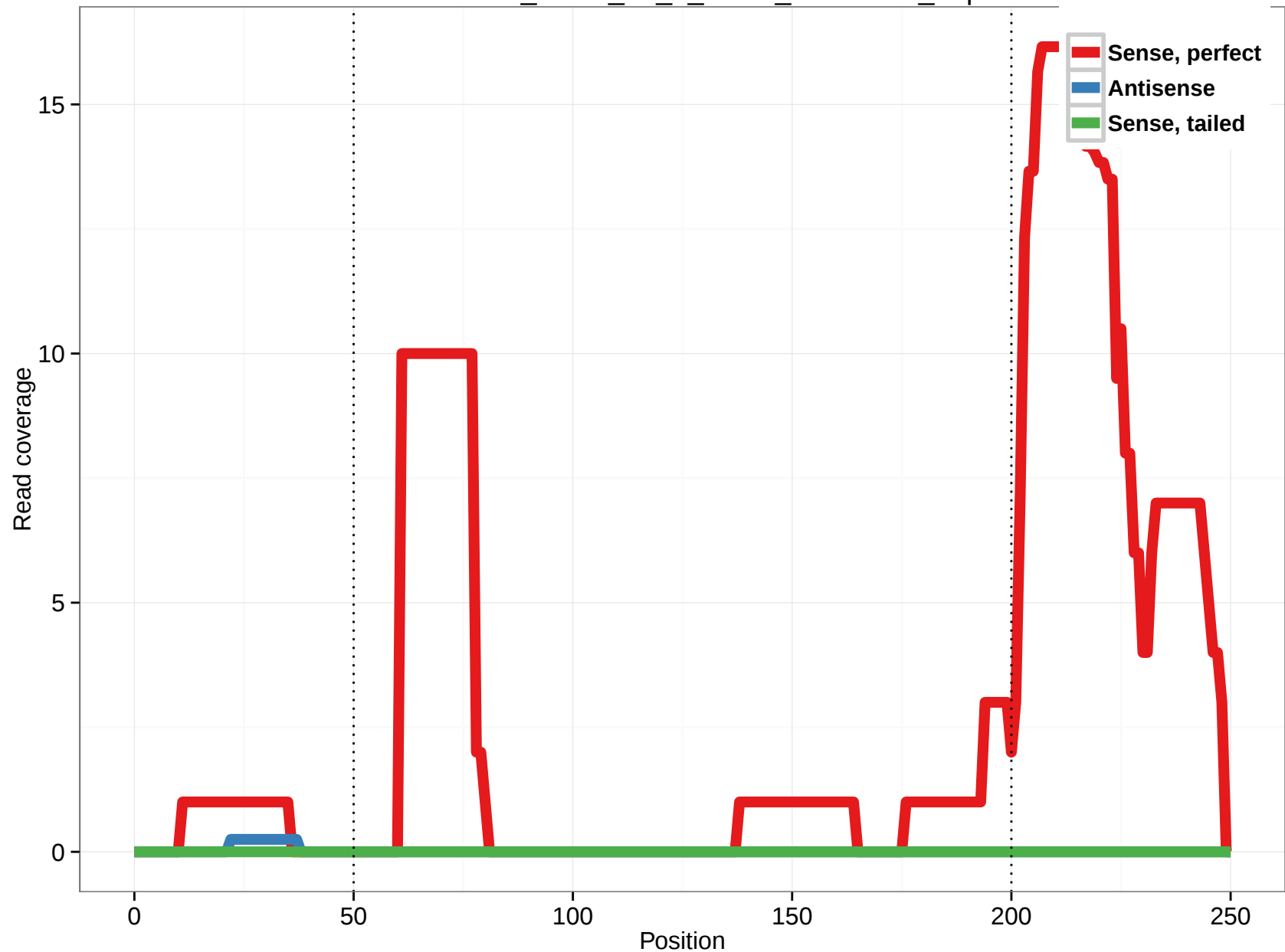
uc010azl.2_intron_23_0_chr15_30058746_r.3p
