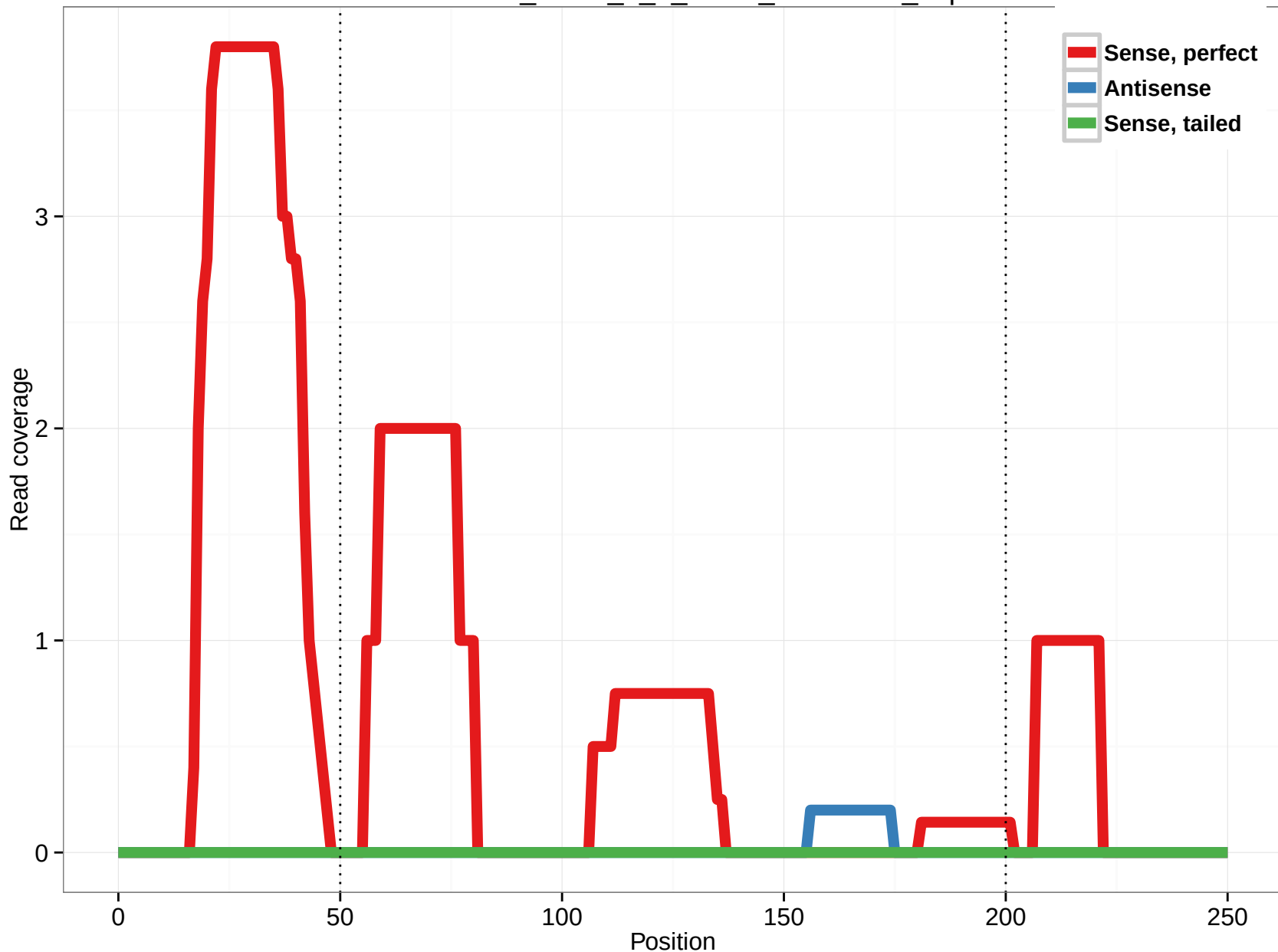
uc010azf.2_intron_1_0_chr15_28986413_f.5p
